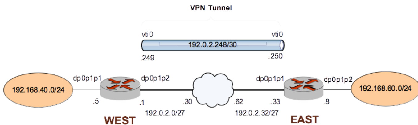
FIGURE 5 IPsec VPN connection with virtual tunnel interfaces
