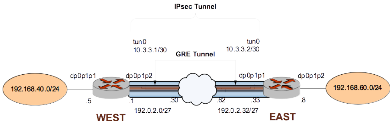
FIGURE 4 GRE tunnel protected by an IPsec tunnel
