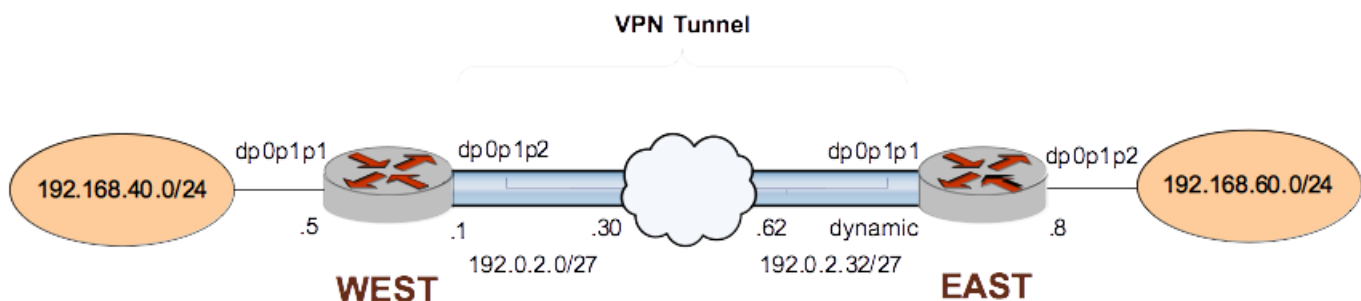
FIGURE 2 IPsec VPN connection with dynamic IP address
