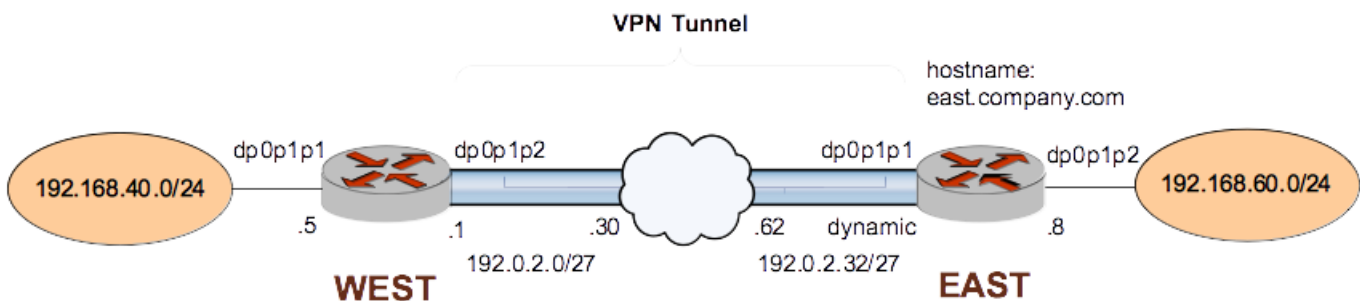
FIGURE 3 IPsec VPN connection with dynamic IP address and dynamic DNS
