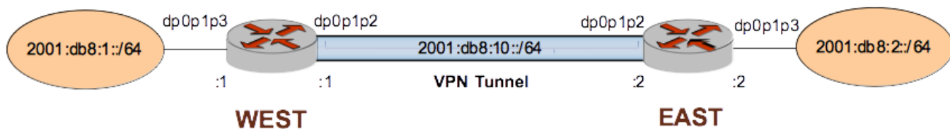
FIGURE 6 Basic site-to-site IPsec VPN connection over IPv6
