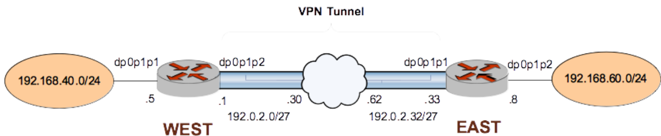
FIGURE 1 Basic site-to-site IPsec VPN connection
