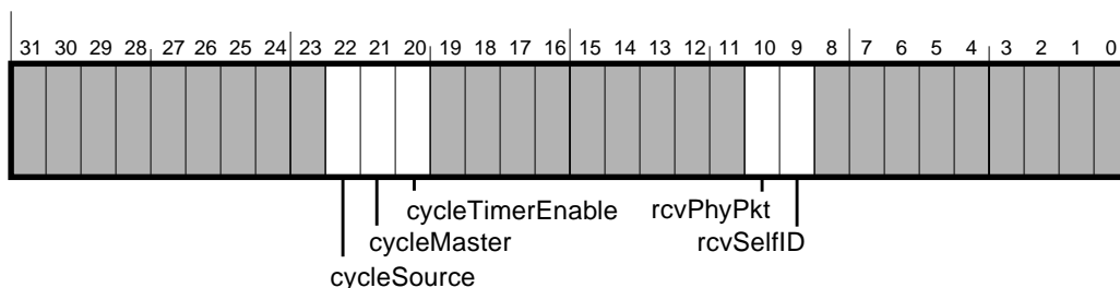
Figure 5-16 — LinkControl register
