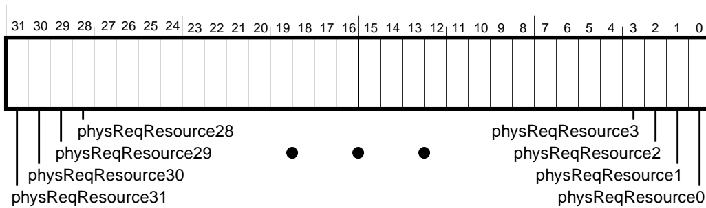
Figure 5-23 — PhysicalRequestFilterLo (set and clear) register
