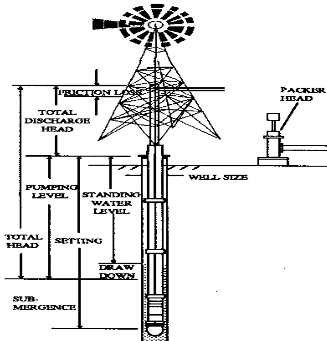
FIGURE 1: Typical Wind Pump
