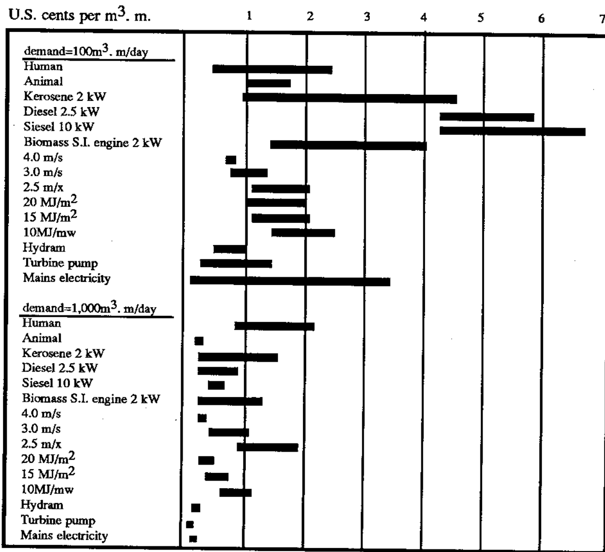
FIGURE 3: Expected range of unit energy costs for two levels of demand, 100 and 1000 m 3 .m/day, for different types of prime mover.
