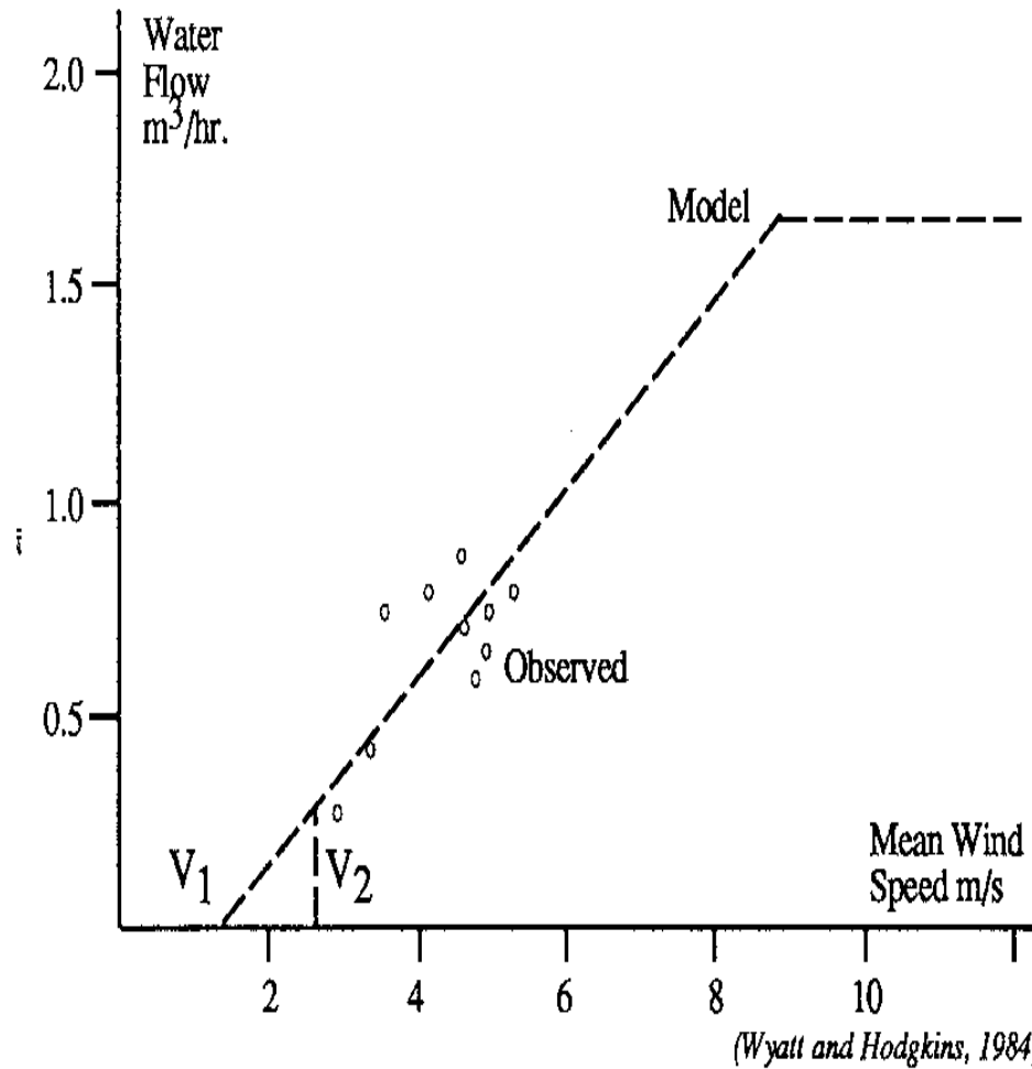
FIGURE 2: Multiblade Windmill Performance, Observed And Model Results, One Minute Average Readings
