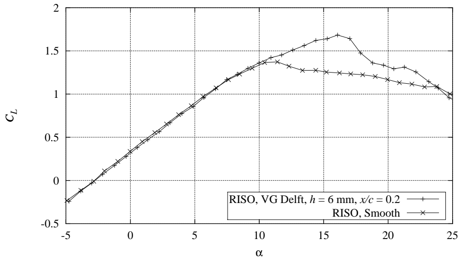
Figure B-3 Measured C_L curve with Delft vortex generators, h = 6 mm, x/c = 0.2 , compared with smooth measurement, Re = 1.6 \times 10^6 , (FFAW3241CONT091297V1).
