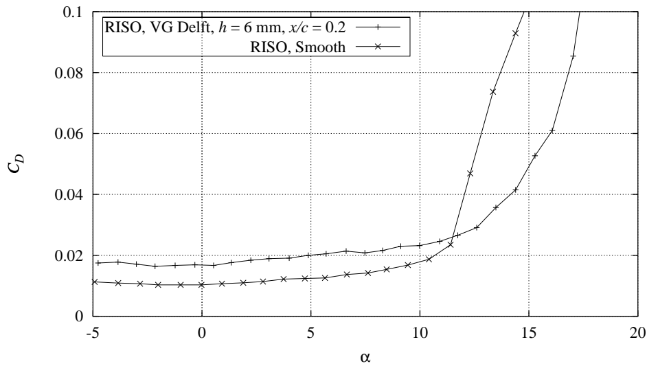
Figure B-4 Measured C_D curve with Delft vortex generators, h = 6 mm, x/c = 0.2 , compared with smooth measurement, Re = 1.6 \times 10^6 , (FFAW3241CONT091297V1).
