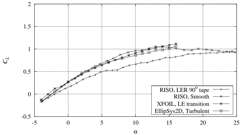
Figure 16-3 Measured C_L curve for 90^\circ zigzag trip tape compared with smooth measurement and XFOIL (LE transition) and EllipSys2D (turbulent) calculations, Re = 1.6 \times 10^6 (NACA63430CONT091297V3).
