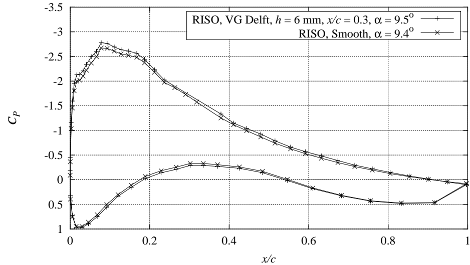
Figure F-7 Measured C_p distribution with Delft vortex generators, h = 6 mm, x/c = 0.3 , compared with smooth measurement, Re = 1.6 \times 10^6 , \alpha = 9.5^\circ (FFAW3301CONT091297V1).
