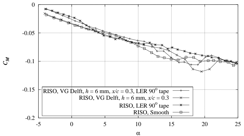
Figure 17-6 Measured C_M curves with combinations of Delft vortex generators, h = 6 \text{ mm} , x/c = 0.3 , and 90^\circ zigzag trip tape compared with smooth measurement, Re = 1.6 \times 10^6 (NACA63430CONT091297V2).
