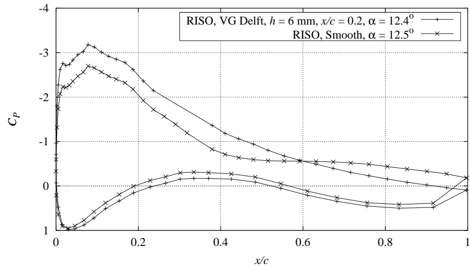
Figure F-8 Measured C_p distribution with Delft vortex generators, h = 6 mm, x/c = 0.2 , compared with smooth measurement, Re = 1.6 \times 10^6 , \alpha = 12.4^\circ (FFAW3301CONT091297V1).
