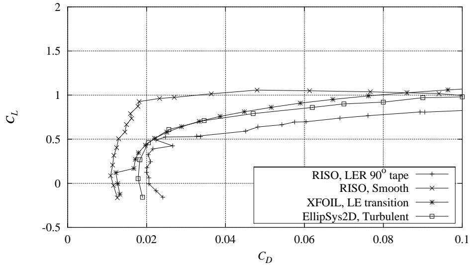
Figure 16-5 Measured C_L - C_D curve for 90^\circ zigzag trip tape compared with smooth measurement and XFOIL (LE transition) and EllipSys2D (turbulent) calculations, Re = 1.6 \times 10^6 (NACA63430CONT091297V3).
