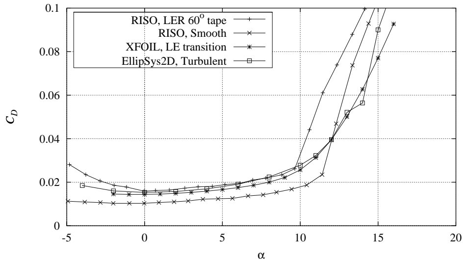
Figure C-10 Measured C_D curve for 60° zigzag trip tape compared with smooth measurement and XFOIL (LE transition) and EllipSys2D (turbulent) calculations, Re = 1.6 \times 10^6 (FFAW3241CONT091297V6).
