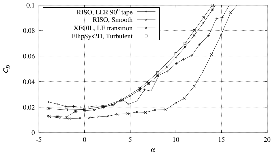
Figure 16-4 Measured C_D curve for 90^\circ zigzag trip tape compared with smooth measurement and XFOIL (LE transition) and EllipSys2D (turbulent) calculations, Re = 1.6 \times 10^6 (NACA63430CONT091297V3).
