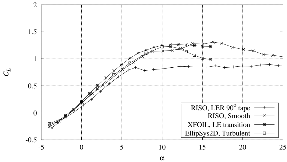
Figure 11-3 Measured C_L curve for 90° zigzag trip tape compared with smooth measurement and XFOIL (LE transition) and EllipSys2D (turbulent) calculations, Re = 1.6 \times 10^6 (FFAW3301CONT091297V3).
