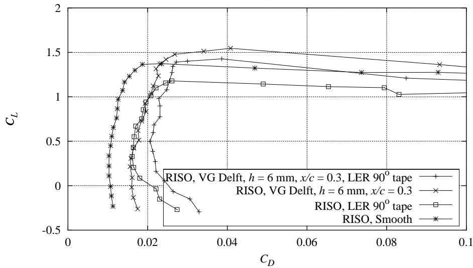
Figure D-5 Measured C_L - C_D curves with combinations of Delft vortex generators, h = 6 \text{ mm} , x/c = 0.3 , and 90^\circ zigzag trip tape compared with smooth measurement, Re = 1.6 \times 10^6 (FFAW3241CONT091297V4).
