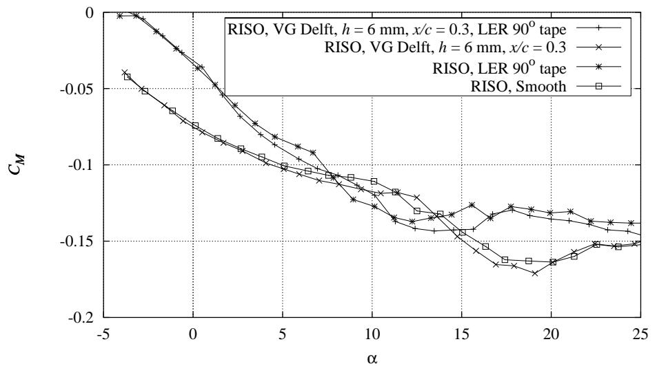
Figure 12-6 Measured C_M curves with combinations of Delft vortex generators, h = 6 \text{ mm} , x/c = 0.3 , and 90^\circ zigzag trip tape compared with smooth measurement, Re = 1.6 \times 10^6 (FFAW3301CONT091297V2).
