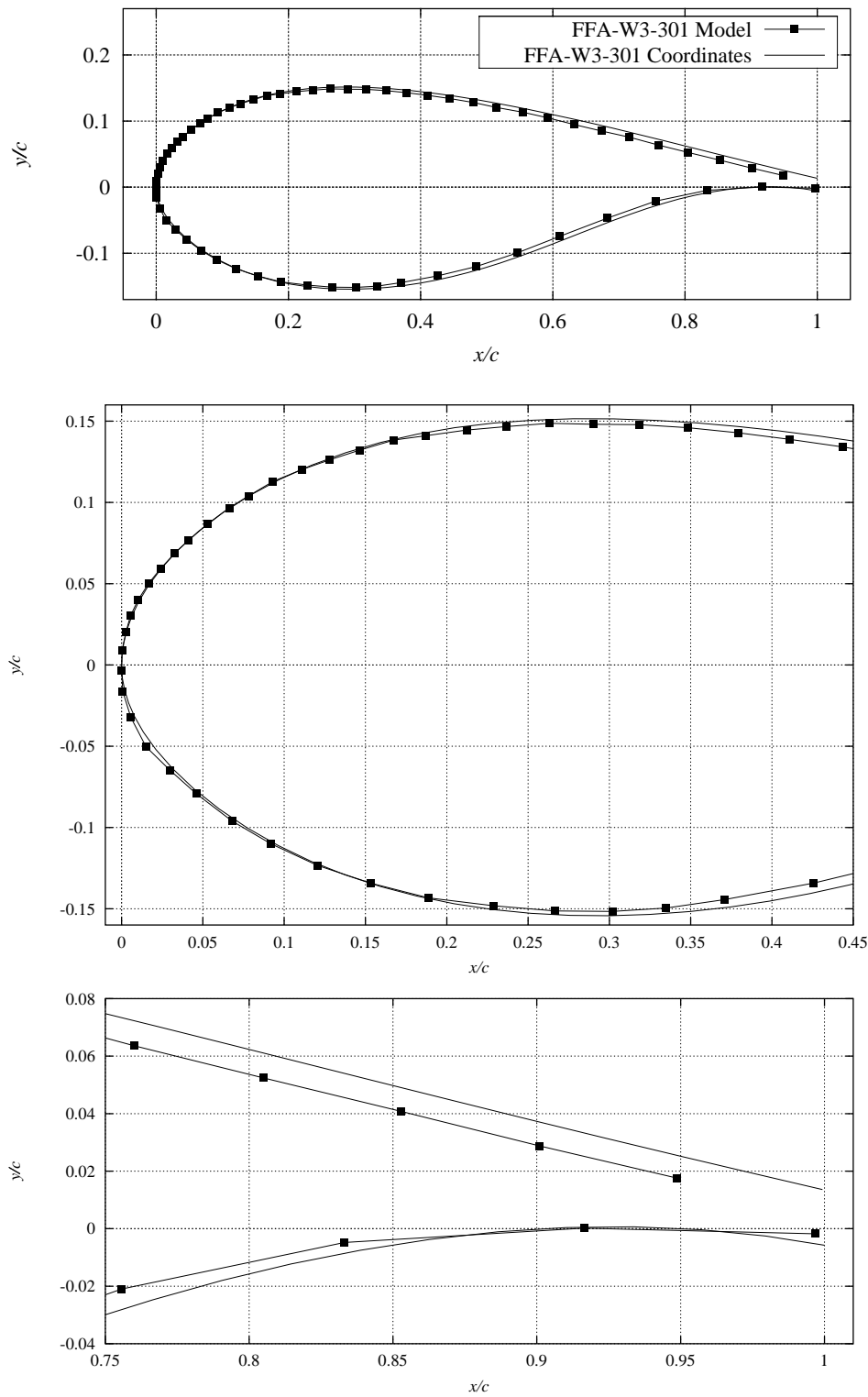
Figure 3-2 The actual FFA-W3-301 model coordinates compared with the theoretical coordinates from [6]. Each symbol corresponds to a pressure tap. The leading edge and the trailing edge regions are shown enlarged.
