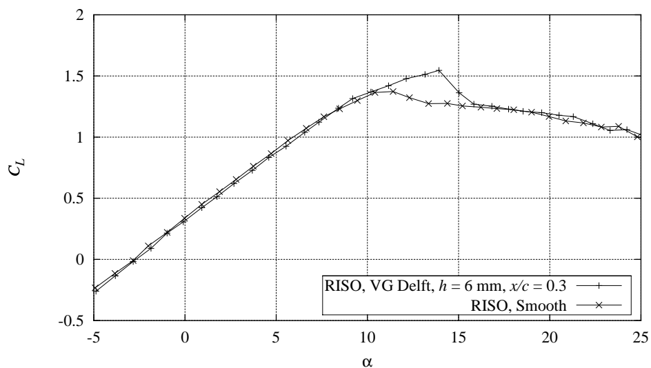
Figure B-9 Measured C_L curve with Delft vortex generators, h = 6 mm, x/c = 0.3 , compared with smooth measurement, Re = 1.6 \times 10^6 (FFAW3241CONT091297V3).
