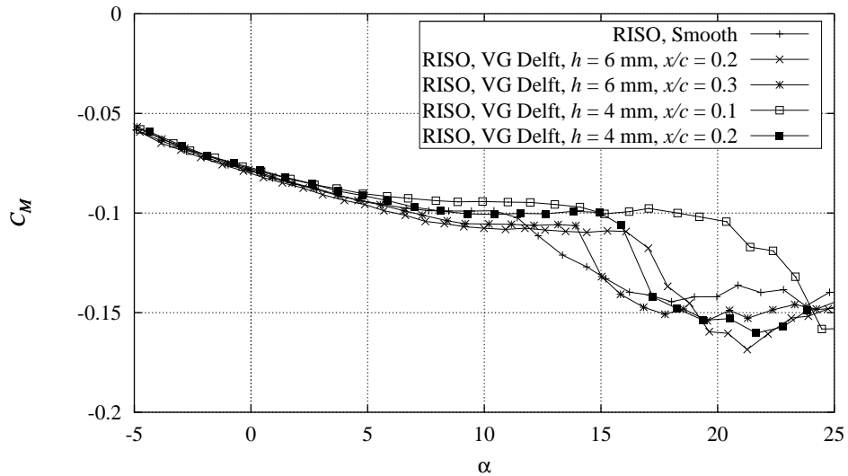
Figure 5-6 Measured C_M curves for the different vortex generator configurations compared with smooth measurement, Re = 1.6 \times 10^6 .
