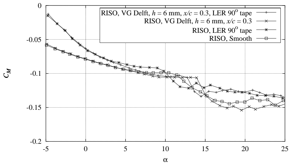
Figure D-6 Measured C_M curves with combinations of Delft vortex generators, h = 6 \text{ mm} , x/c = 0.3 , and 90^\circ zigzag trip tape compared with smooth measurement, Re = 1.6 \times 10^6 (FFAW3241CONT091297V4).
