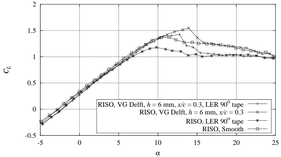
Figure D-3 Measured C_L curves with combinations of Delft vortex generators, h = 6 mm, x/c = 0.3 , and 90^\circ zigzag trip tape compared with smooth measurement, Re = 1.6 \times 10^6 (FFAW3241CONT091297V4).
