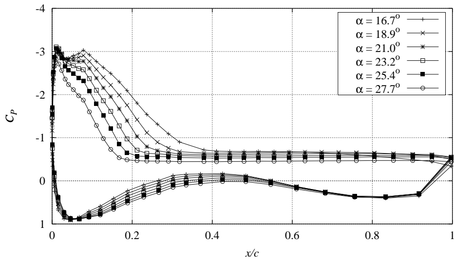
Figure 9-1 Measured C_p distributions at different angles of attack (FFAW3301STEP091297V1).
