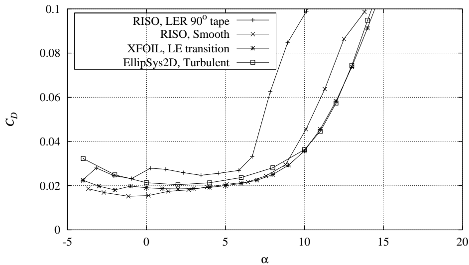
Figure 11-4 Measured C_D curve for 90° zigzag trip tape compared with smooth measurement and XFOIL (LE transition) and EllipSys2D (turbulent) calculations, Re = 1.6 \times 10^6 (FFAW3301CONT091297V3).
