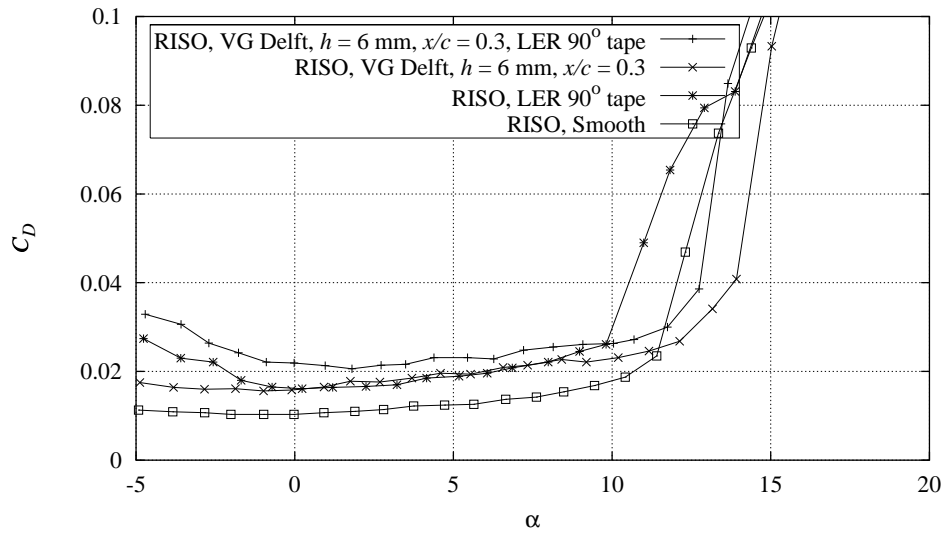
Figure D-4 Measured C_D curves with combinations of Delft vortex generators, h = 6 mm, x/c = 0.3 , and 90^\circ zigzag trip tape compared with smooth measurement, Re = 1.6 \times 10^6 (FFAW3241CONT091297V4).
