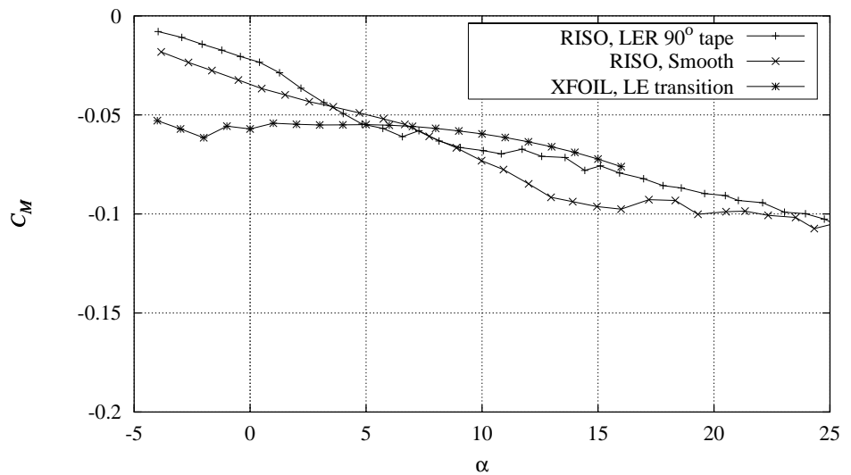
Figure 16-6 Measured C_M curve for 90^\circ zigzag trip tape compared with smooth measurement and XFOIL (LE transition) calculations, Re = 1.6 \times 10^6 (NACA63430CONT091297V3).
