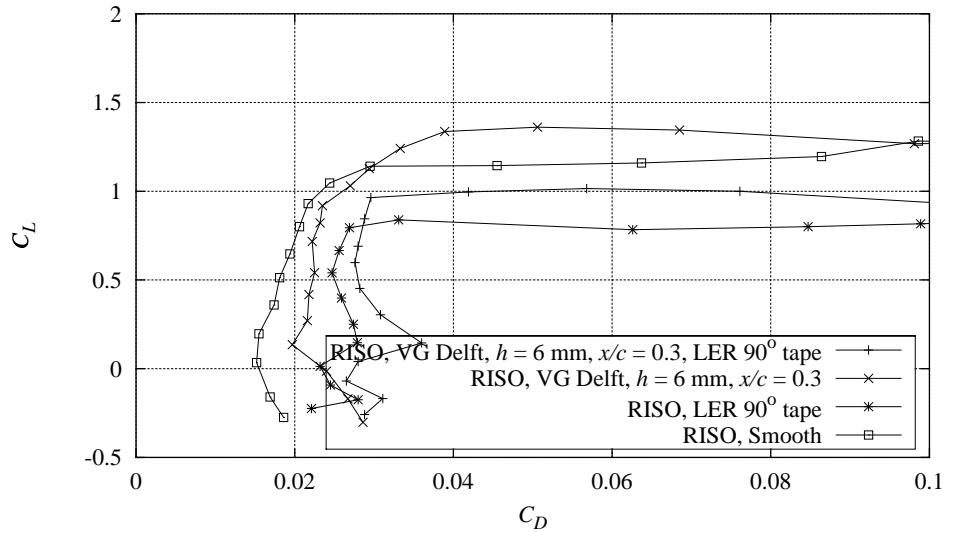
Figure 12-5 Measured C_L - C_D curves with combinations of Delft vortex generators, h = 6 \text{ mm} , x/c = 0.3 , and 90^\circ zigzag trip tape compared with smooth measurement, Re = 1.6 \times 10^6 (FFAW3301CONT091297V2).
