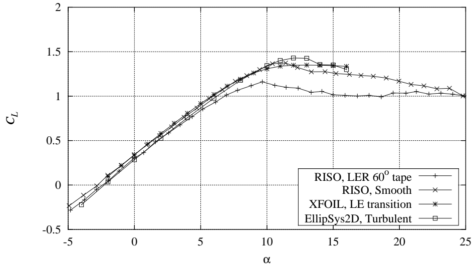
Figure C-9 Measured C_L curve for 60° zigzag trip tape compared with smooth measurement and XFOIL (LE transition) and EllipSys2D (turbulent) calculations, Re = 1.6 \times 10^6 (FFAW3241CONT091297V6).
