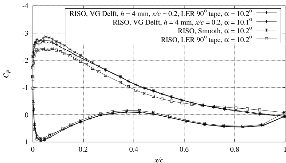
Figure D-7 Measured C_p distributions with combinations of Delft vortex generators, h = 4 mm, x/c = 0.2 , and 90^\circ zigzag trip tape compared with smooth measurement, Re = 1.6 \times 10^6 , \alpha around 10^\circ (FFAW3241CONT091297V8).
