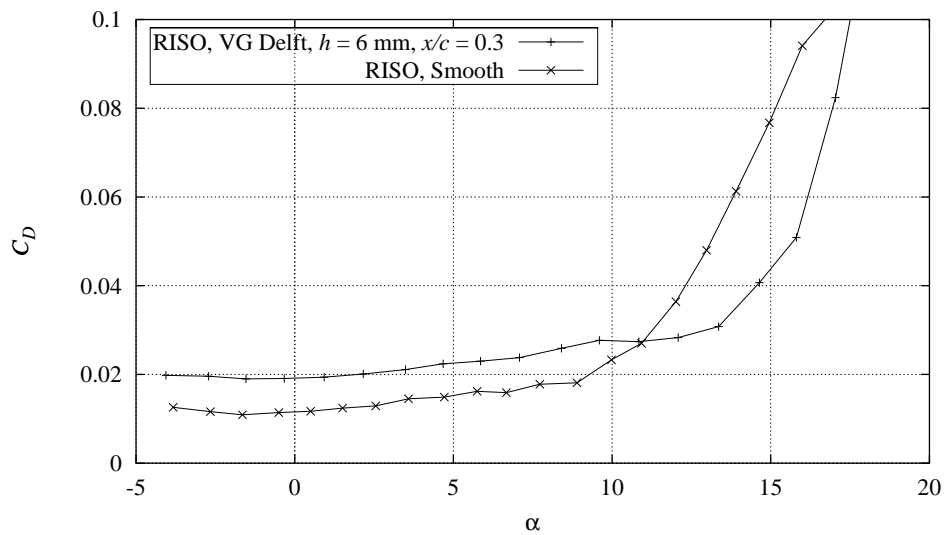
Figure H-10 Measured C_D curve with Delft vortex generators, h = 6 mm, x/c = 0.3 , compared with smooth measurement, Re = 1.6 \times 10^6 , (NACA63430CONT091297V1).
