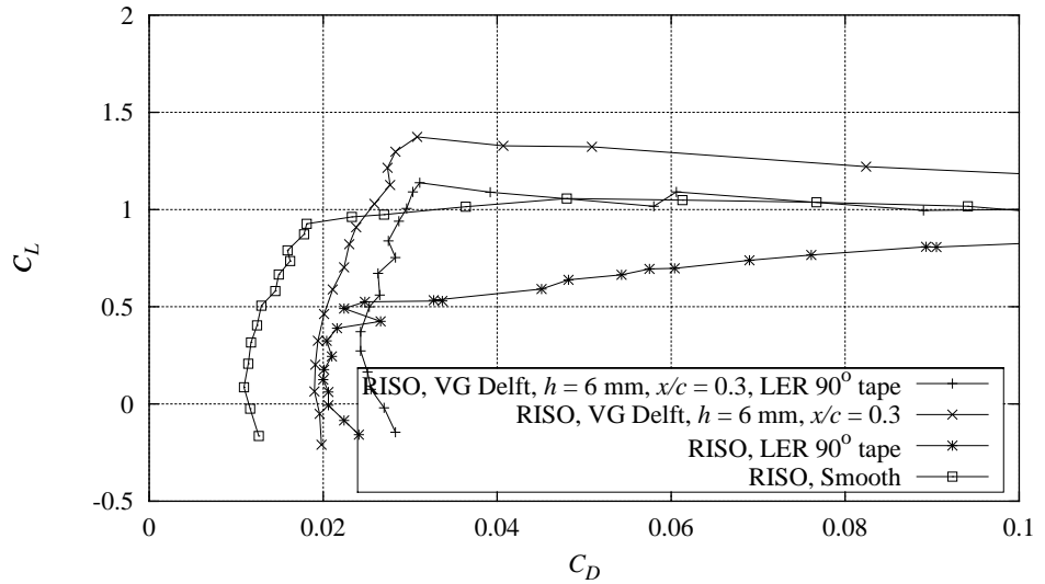
Figure 17-5 Measured C_L - C_D curves with combinations of Delft vortex generators, h = 6 \text{ mm} , x/c = 0.3 , and 90^\circ zigzag trip tape compared with smooth measurement, Re = 1.6 \times 10^6 (NACA63430CONT091297V2).
