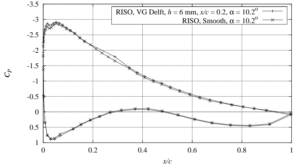
Figure B-1 Measured C_p distribution with Delft vortex generators, h = 6 mm, x/c = 0.2 , compared with smooth measurement, Re = 1.6 \times 10^6 , \alpha = 10.2^\circ (FFAW3241CONT091297V1).
