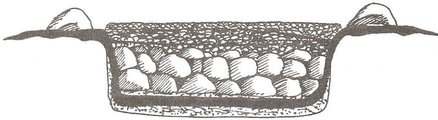
Figure 4.5 A cross section of the foundation
