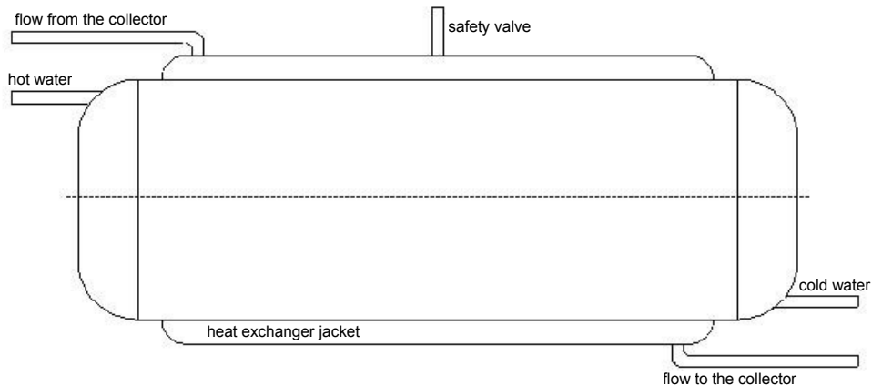
Fig. 6: Drawing of a hot water tank
