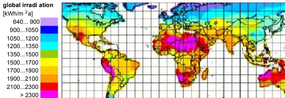
Fig. 1: Global irradiation in kWh/m 2 a [7]
