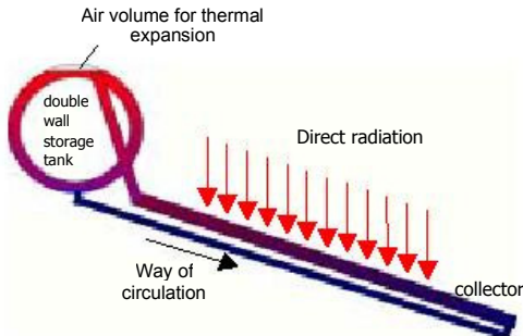
Fig. 2: Gross section of a SWH.
