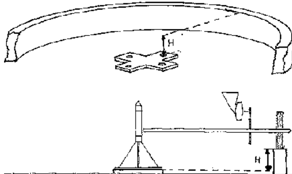
Fig. 31: Determination of the foundation height
