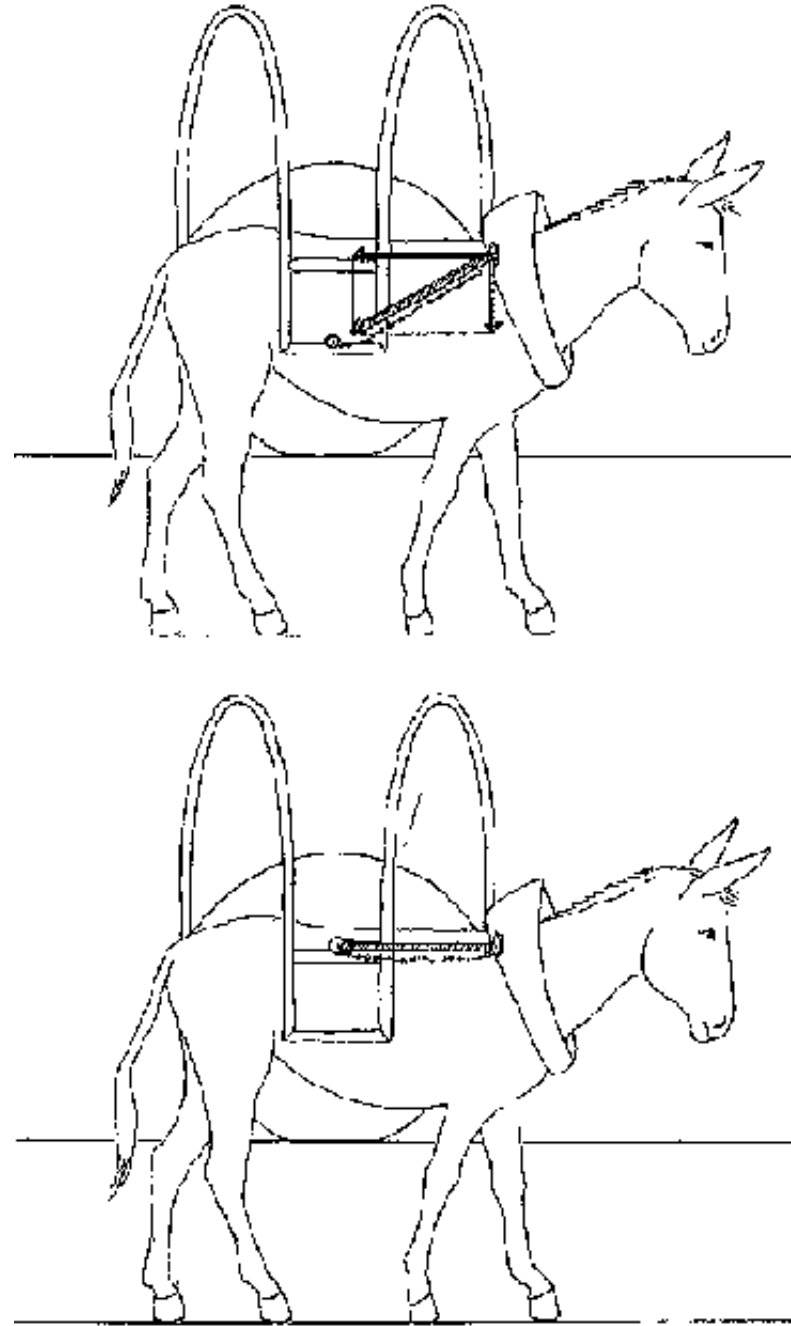
Fig. 16: Vertical and horizontal components of the tractive power; no power losses
