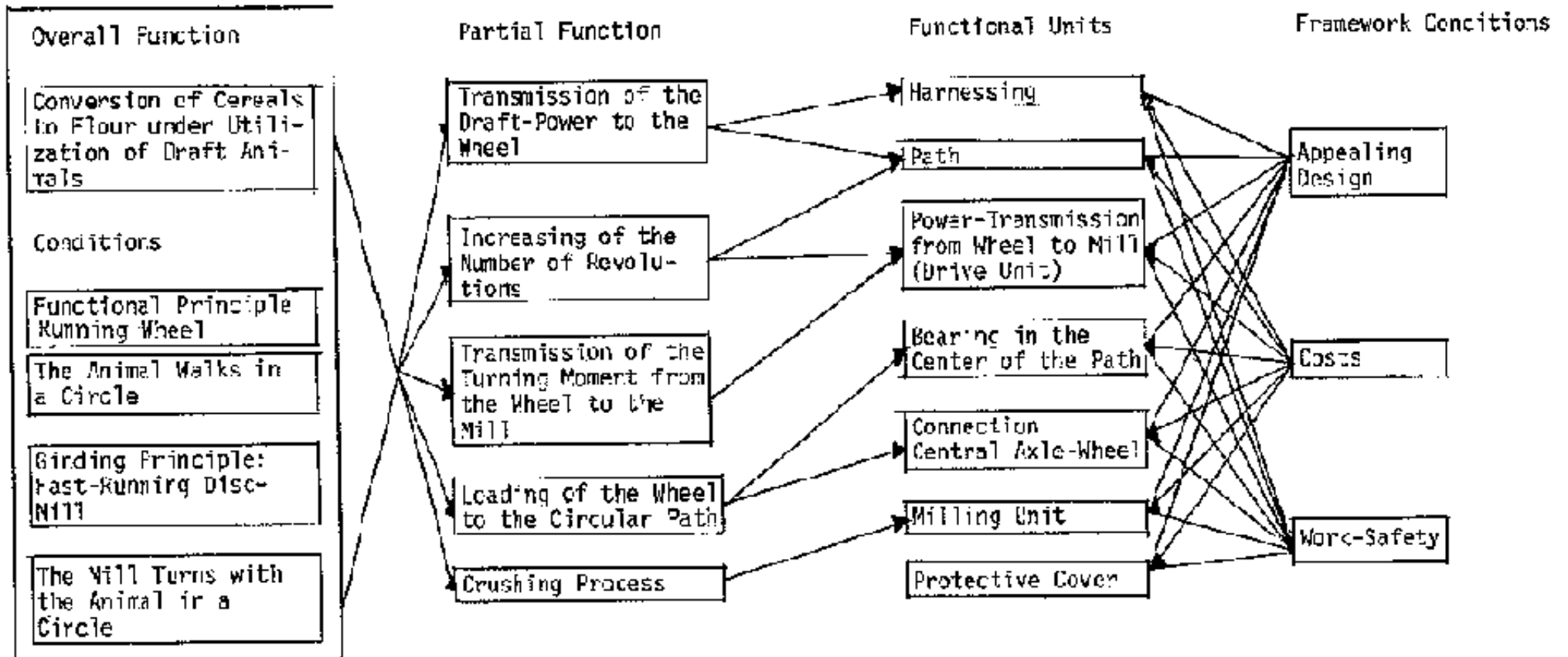
FIGURE 12: Functional diagram of the animal powered mill.
