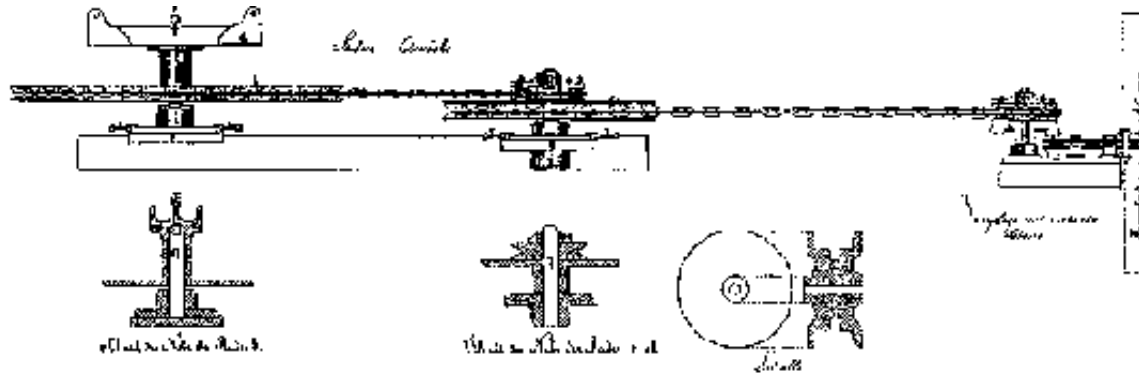
Fig. 3: A "chain power gear" patented in the German Reich in 1879
