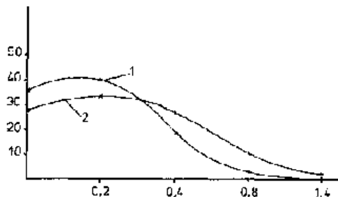
Fig. 2: (1) Particle-size distribution curve of a flour type, which is suitable for the preparation of the millet dish To according to a Mali housewife (2) Particle-size distribution curve of a flour suitable for the preparation of couscous, according to the same housewife.
