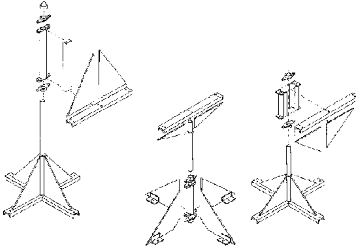
Fig. 32: Different constructions of the central axle
