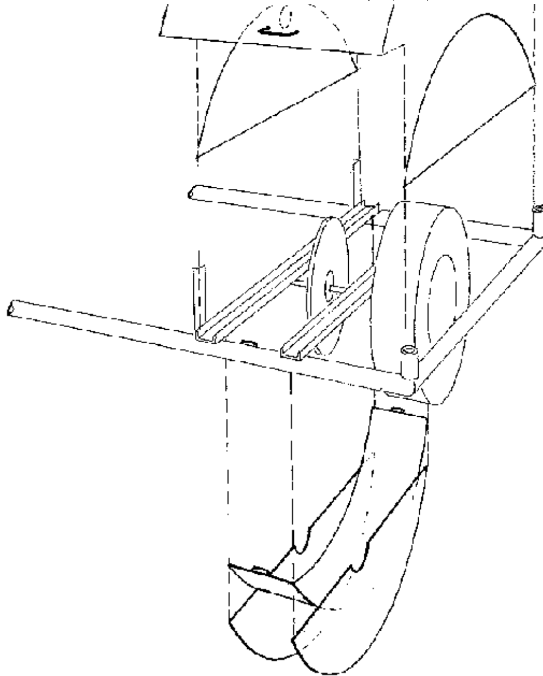
Fig 38: Arrangement of the protective coverings on the frame
