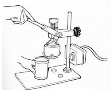
Fig. 1. Yoghurt pot sealer. (Practical Action)
