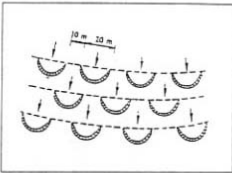
Figure 5: RWH with semi-circular bunds: http://www.fao.org/ag/ags/agse/3ero/namibia1/c21.htm
