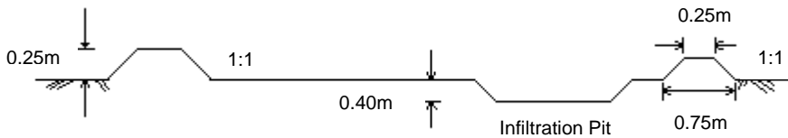
Figure 4: Cross section of catchment area.
