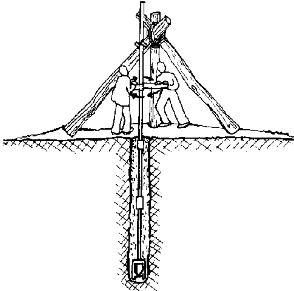
FIG. 11-3. HAND AUGERING
