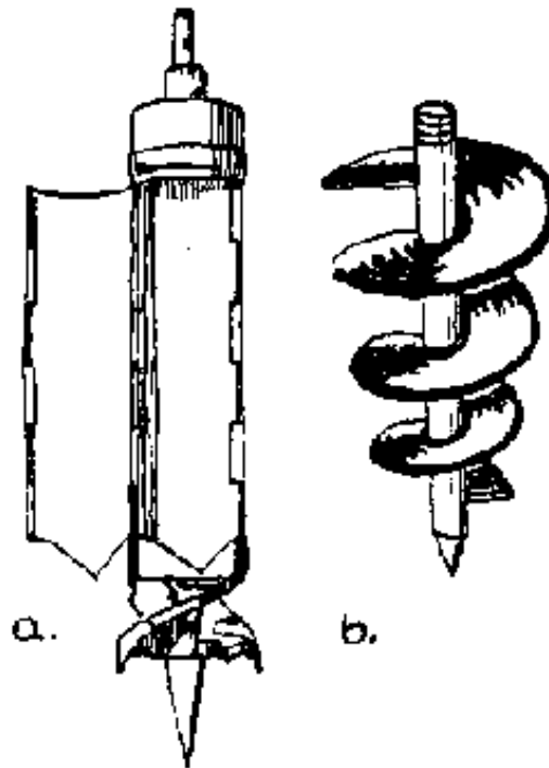
FIG. 10-4. AUGER BITS.
