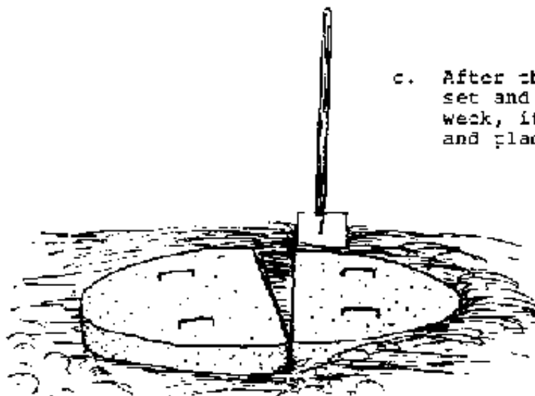
FIG. 9-10. CASTING THE BOTTOM PLUG
