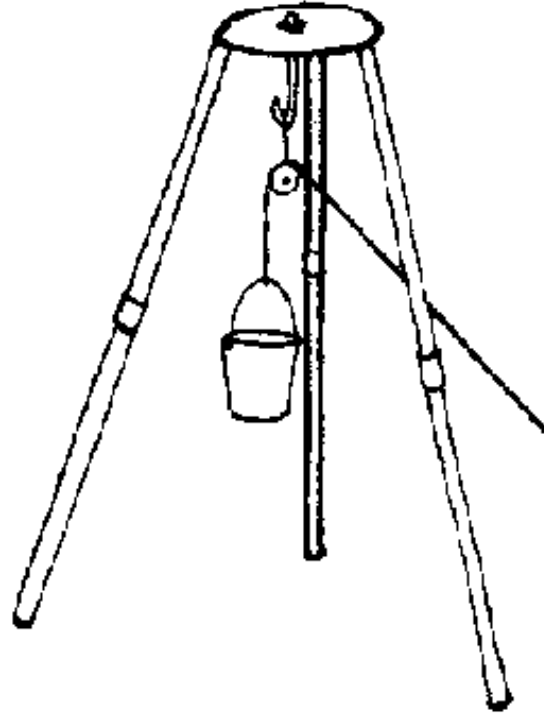
FIG. 5-5. TRIPOD
