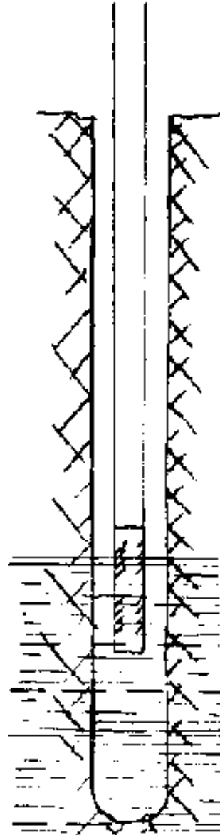
FIG. 15-7. SCREEN AND CASING LOWERED INTO COMPLETED
