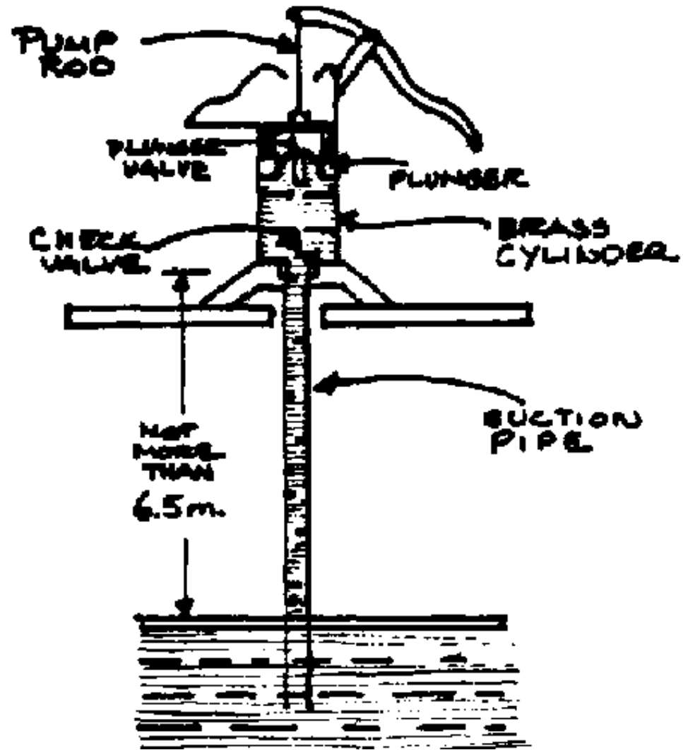
FIG. VII-2. SHALLOW WELL LIFT PUMP
