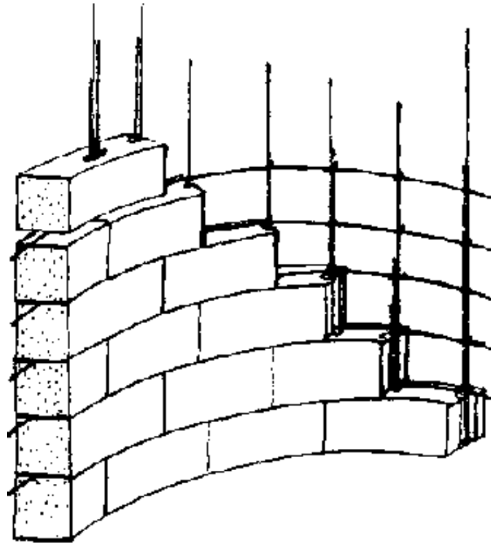
FIG. 8-15. REINFORCED BRICK LINING
