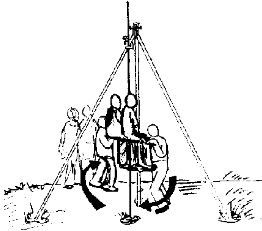
FIG. 12-5. ADDED WEIGHT NECESSARY TO PENETRATE HARD GROUND
