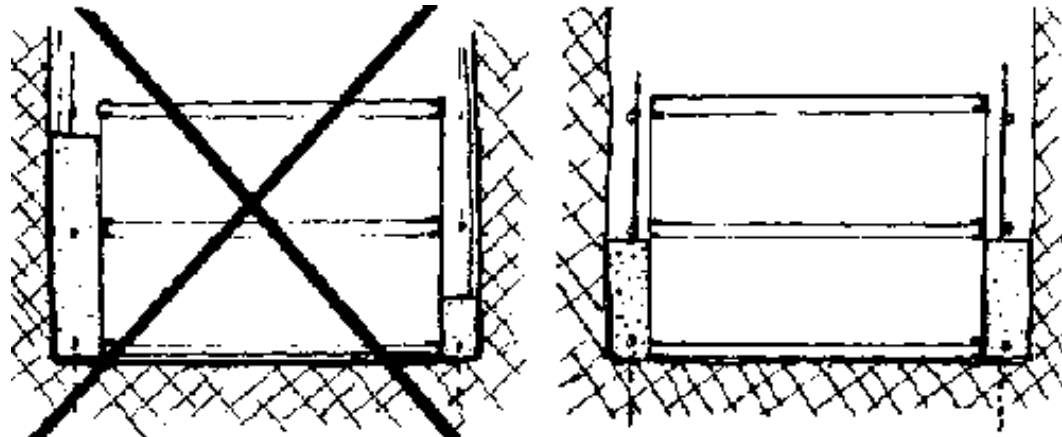
FIG. 8-5. POURING CONCRETE EVENLY IN PLACE AROUND MOLD.
