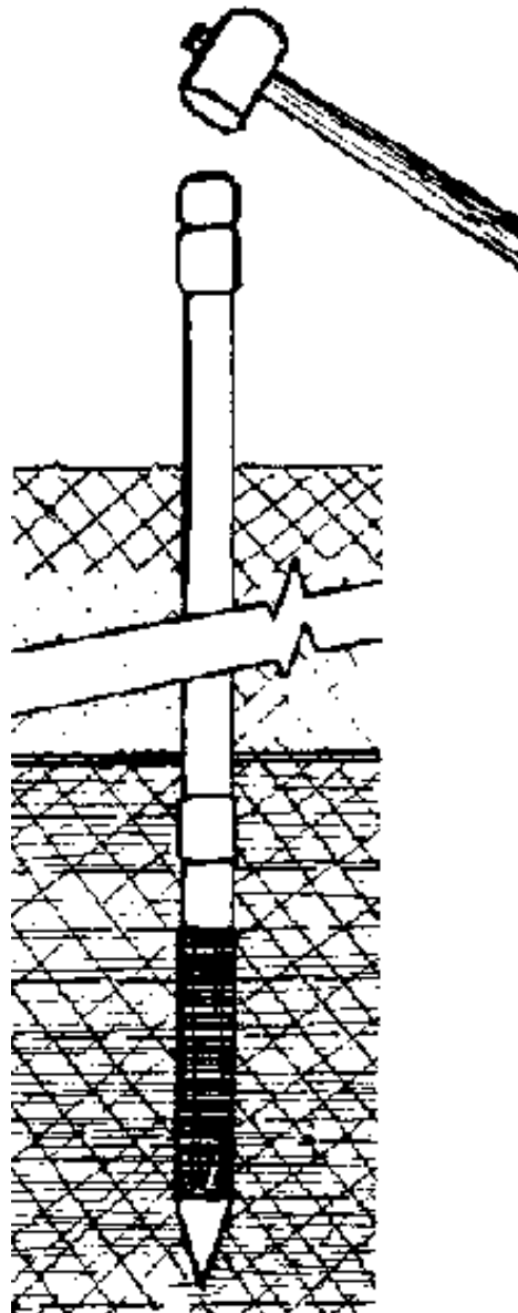
FIG. 11-7. DRIVEN WELL
