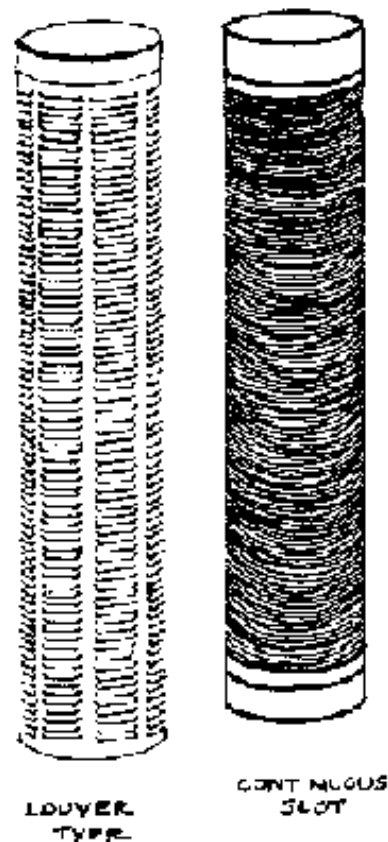
FIG. 15-1. MANUFACTURED SCREENS
