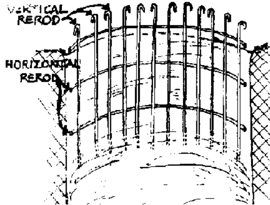
FIG. 8-1. REINFORCED CONCRETE LINING BUILT IN PLACE (a)
