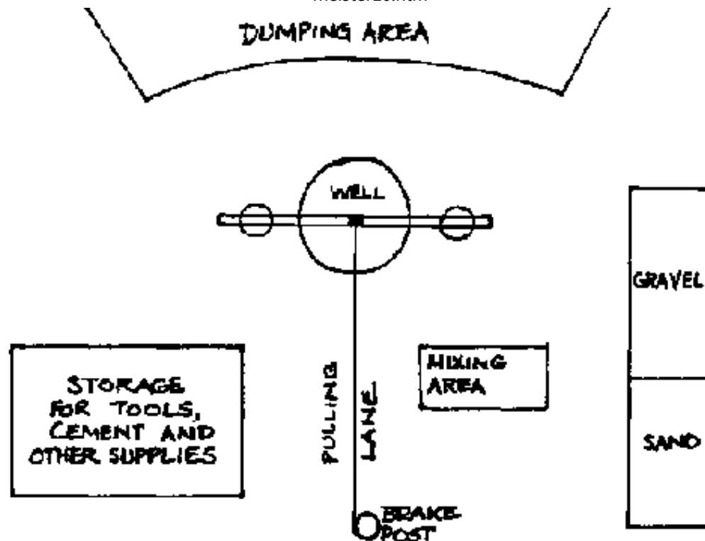
FIG. 4-1. LAYOUT OF MATERIALS AND SUPPLIES
