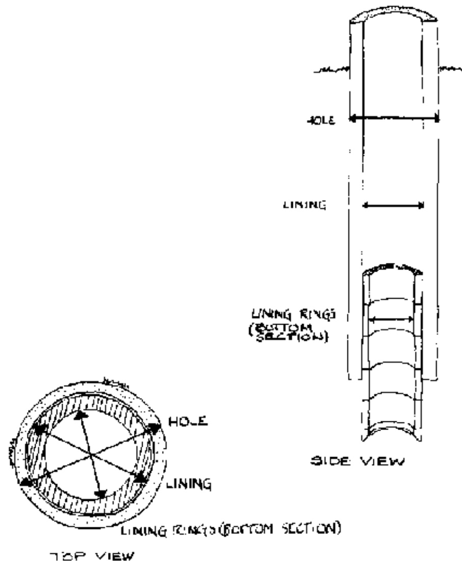
FIG. 3-4. THREE DIFFERENT WELL DIAMETERS USED DURING CONSTRUCTION
