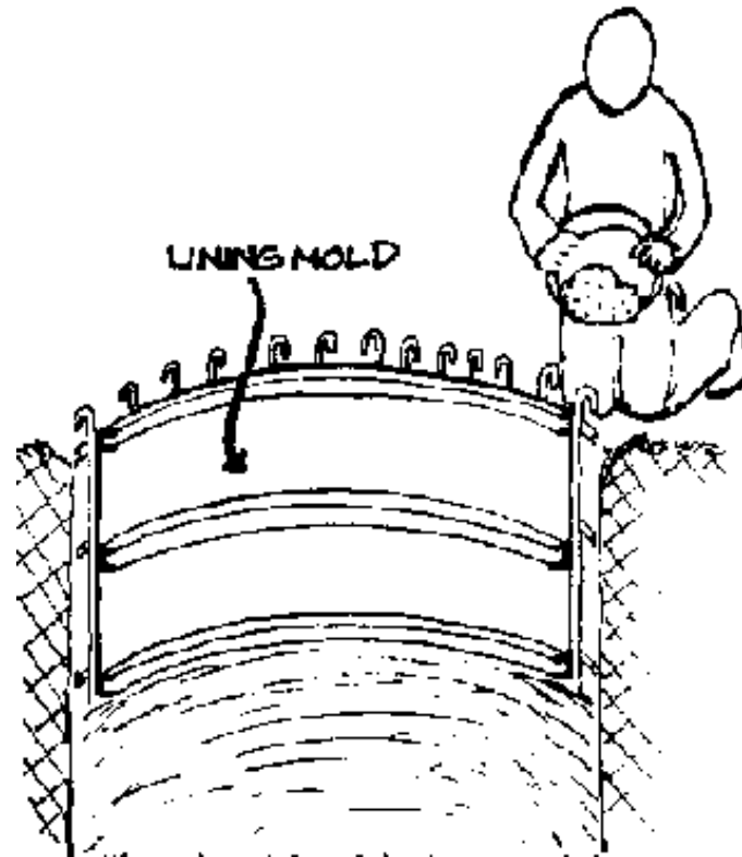
FIG. 8-1. REINFORCED CONCRETE LINING BUILT IN PLACE (b)
