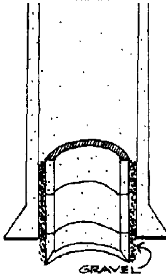
FIG. 9-5. GRAVEL USED TO GUIDE SINKING RINGS
