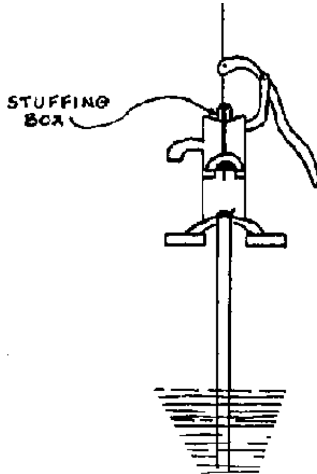
FIG. VII-4. SHALLOW WELL; LIFT AND FORCE PUMP
