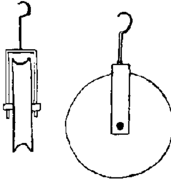
FIG. 5-13. PULLEY WITH MOUNTING HOOK
