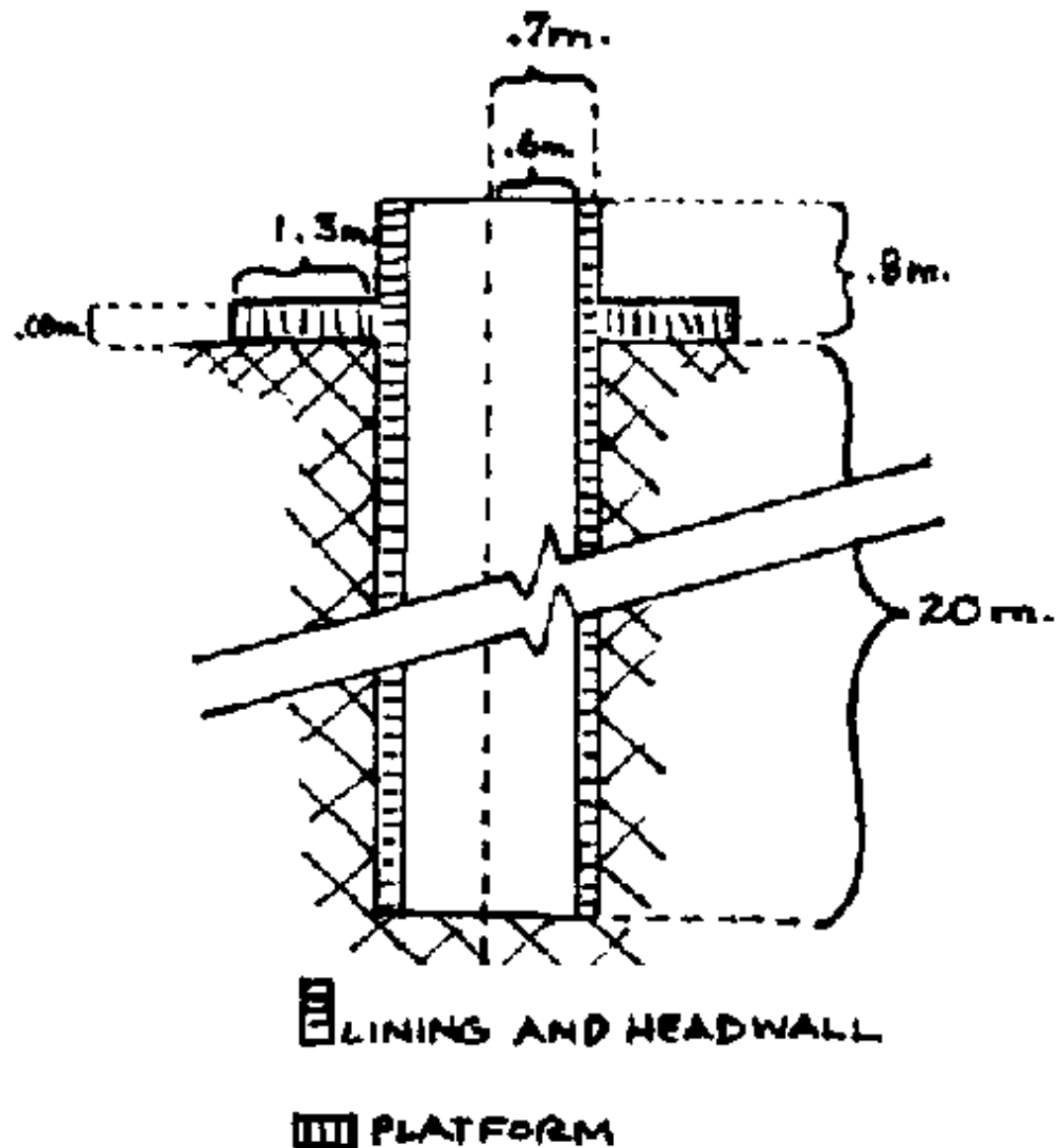
FIG. IV-1. CROSS SECTION OF TYPICAL WELL FOR CALCULATION OF CONCRETE NEEDS
