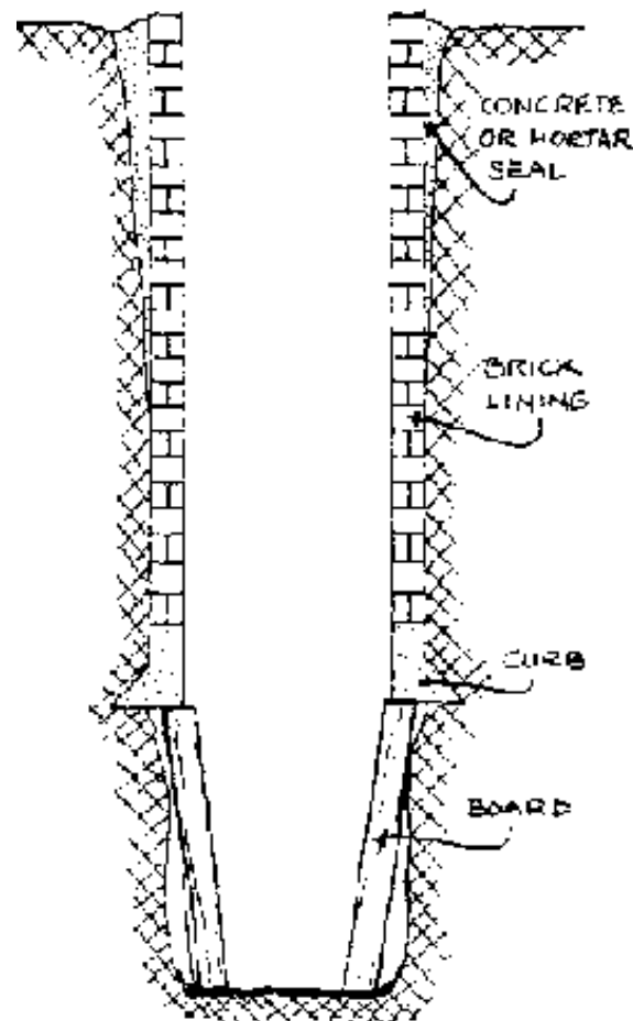
FIG. 8-16. SECTION OF BRICK LINING
