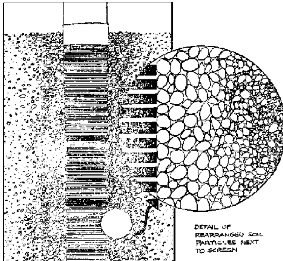
FIG. 10-5. CONTINUOUS SLOT WELL SCREEN IN DEVELOPED GROUND FORMATION
