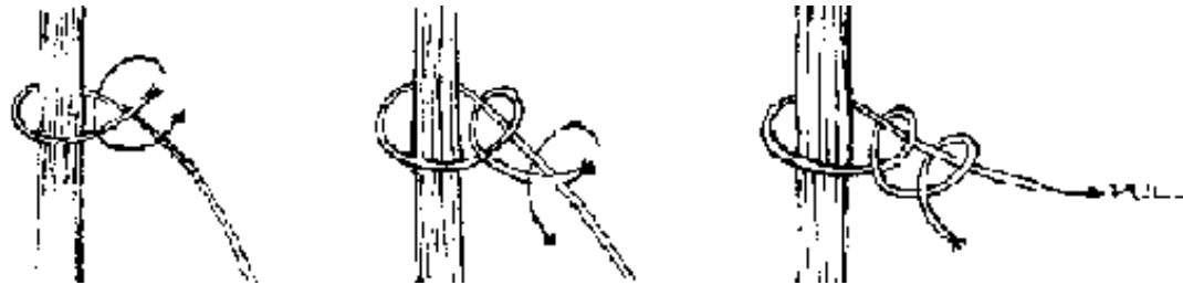
FIG. 5-11. HALF HITCHES
