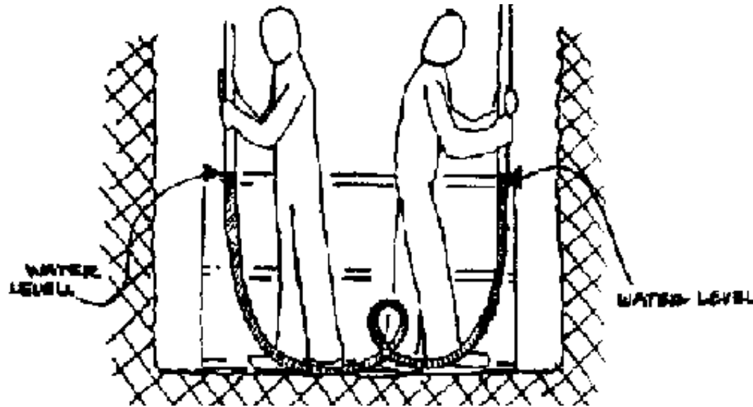
FIG. V-4. CLEAR HOSE AND WATER USED AS LEVEL
