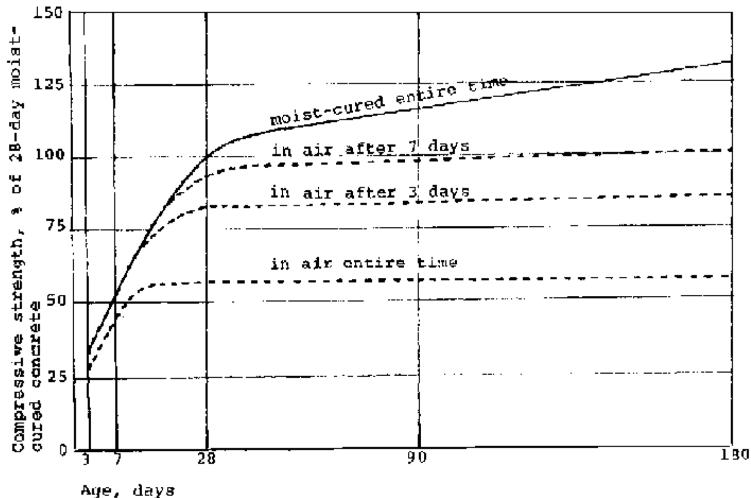
GRAPH: STRENGTH OF CONCRETE AFTER DAYS OF MOIST-CURING
