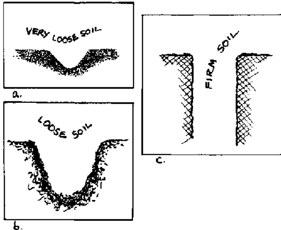
FIG. 3 -5. GROUND CONDITIONS
