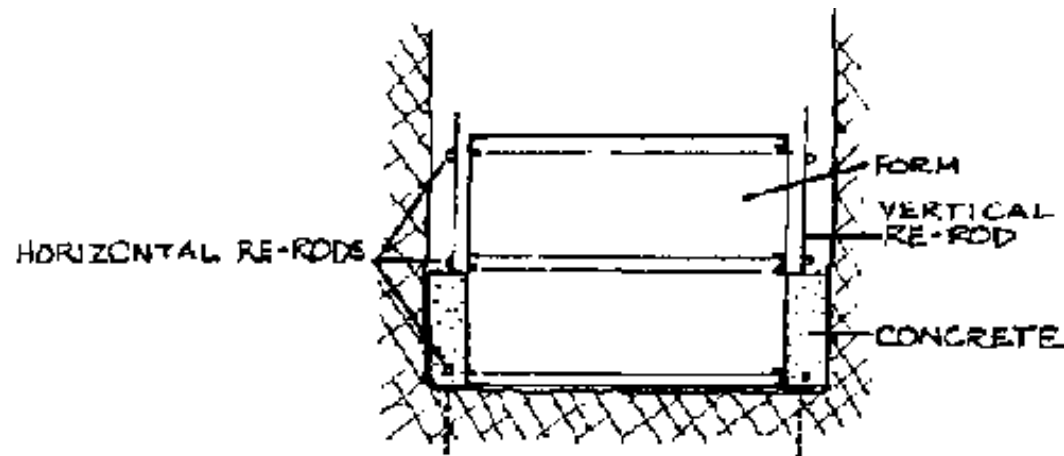
FIG. IV-2. INTERIOR LINING FORM
