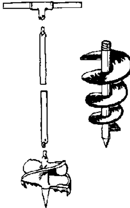
FIG. 12-3. OPEN BLADE AUGERS
