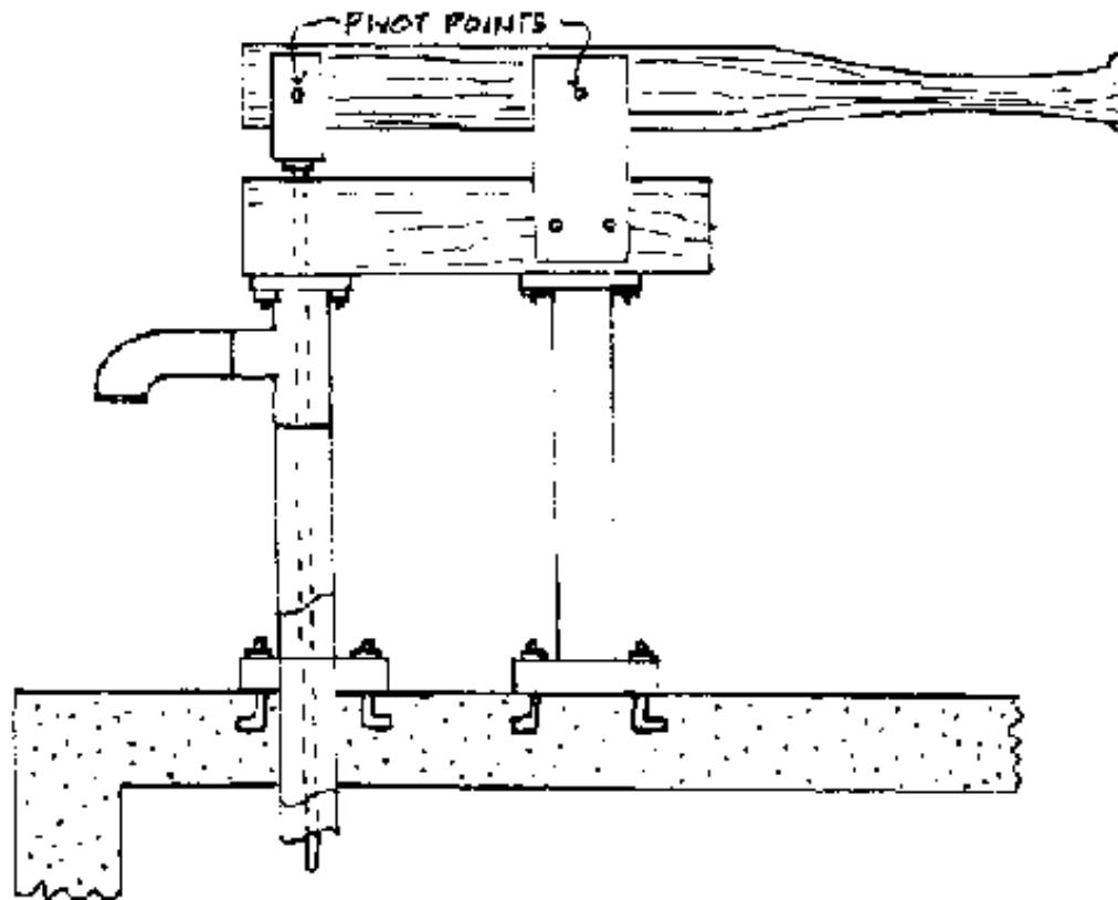
FIG. VII-15. LOCALLY MADE PUMP HEAD
