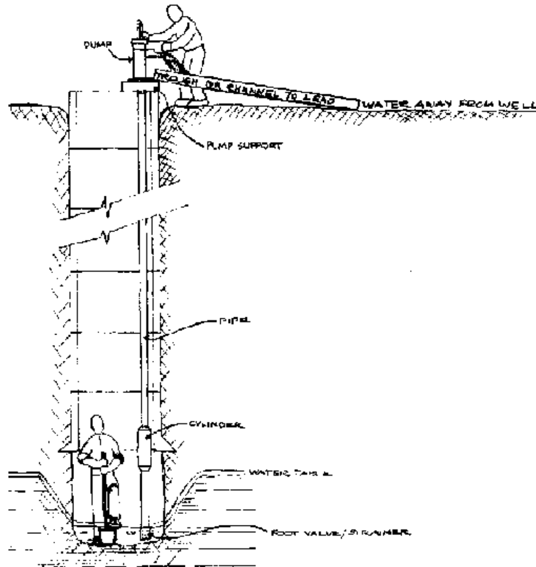
FIG. 9-1. USING A PUMP TO REMOVE WATER FROM BOTTOM SECTION WHILE SINKING
