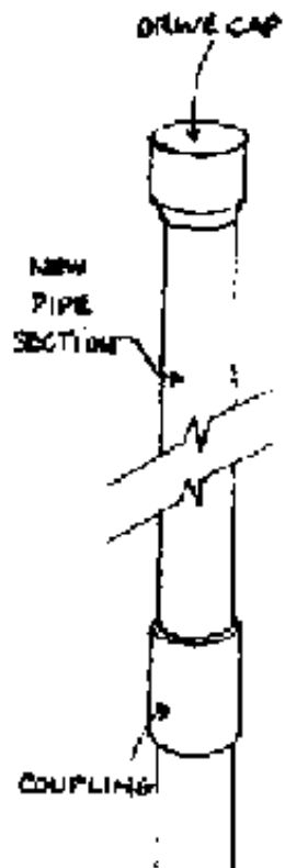
FIG. 14-9. INSTALLING NEW PIPE SECTION
