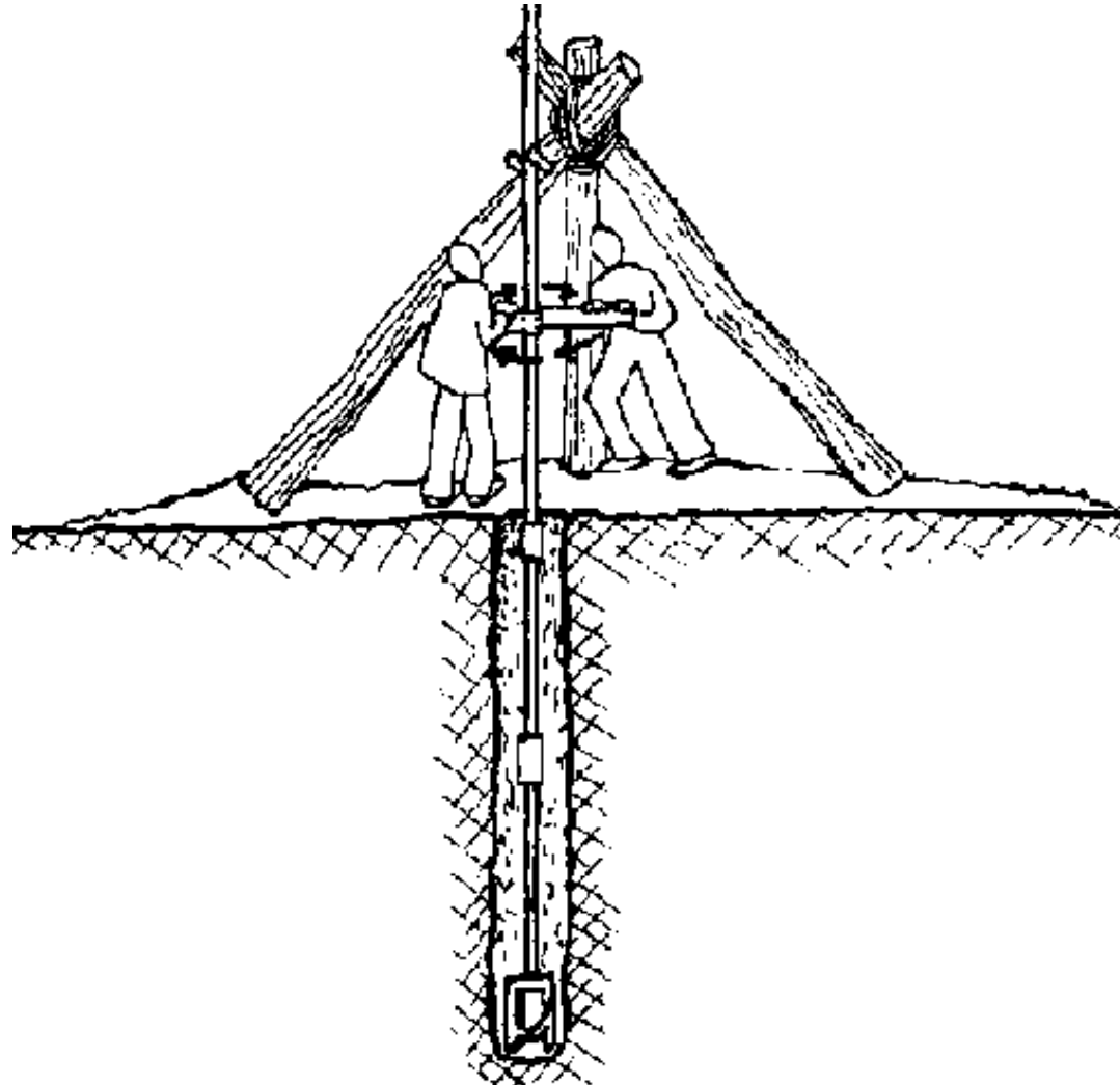
FIG. 1-4. DRILLING A WELL
