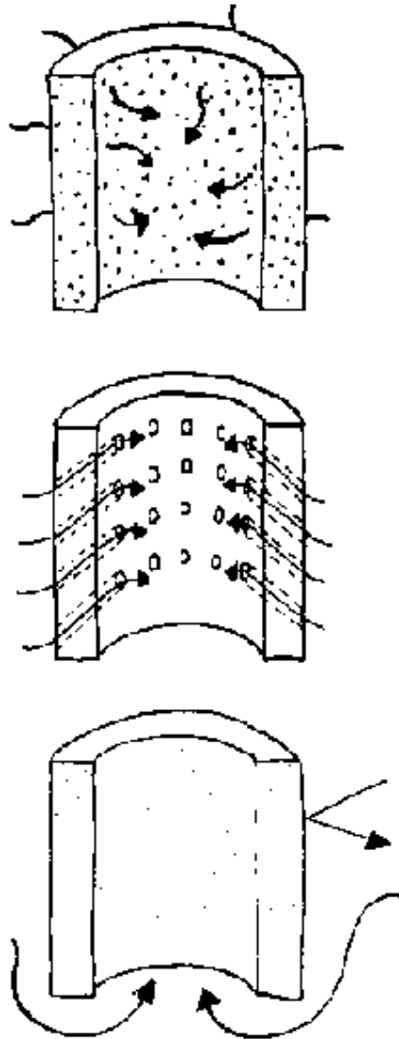
FIG. 3-6. WATER ENTRY INTO WELL
