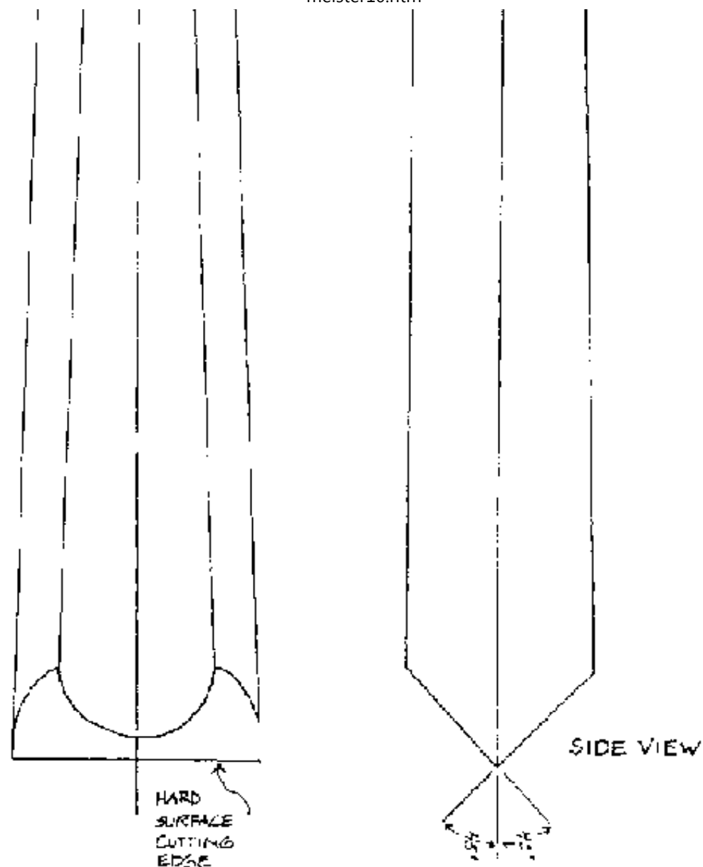
FIG. 12-9. DETAIL OF PERCUSSION BIT
