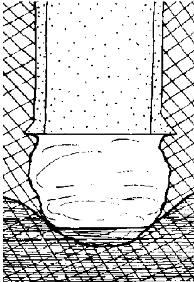
FIG. 9-2. HOLE WALLS COLLAPSING IN BOTTOM SECTION
