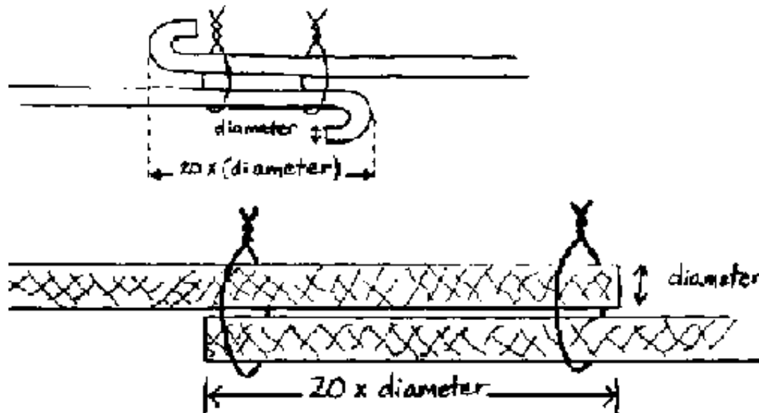
FIG. IV-4. REROD OVERLAP
