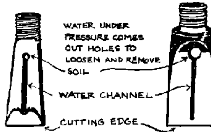
FIG. 14-12. JETTING BITS
