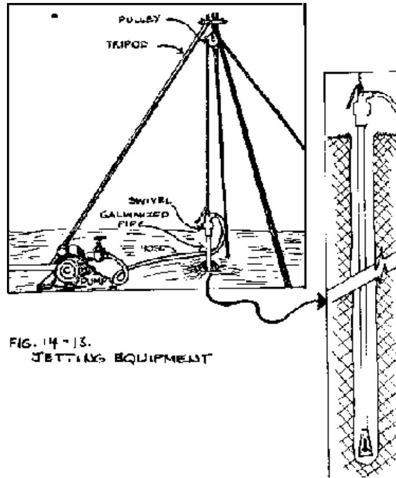
FIG. 14-13. JETTING EQUIPMENT
