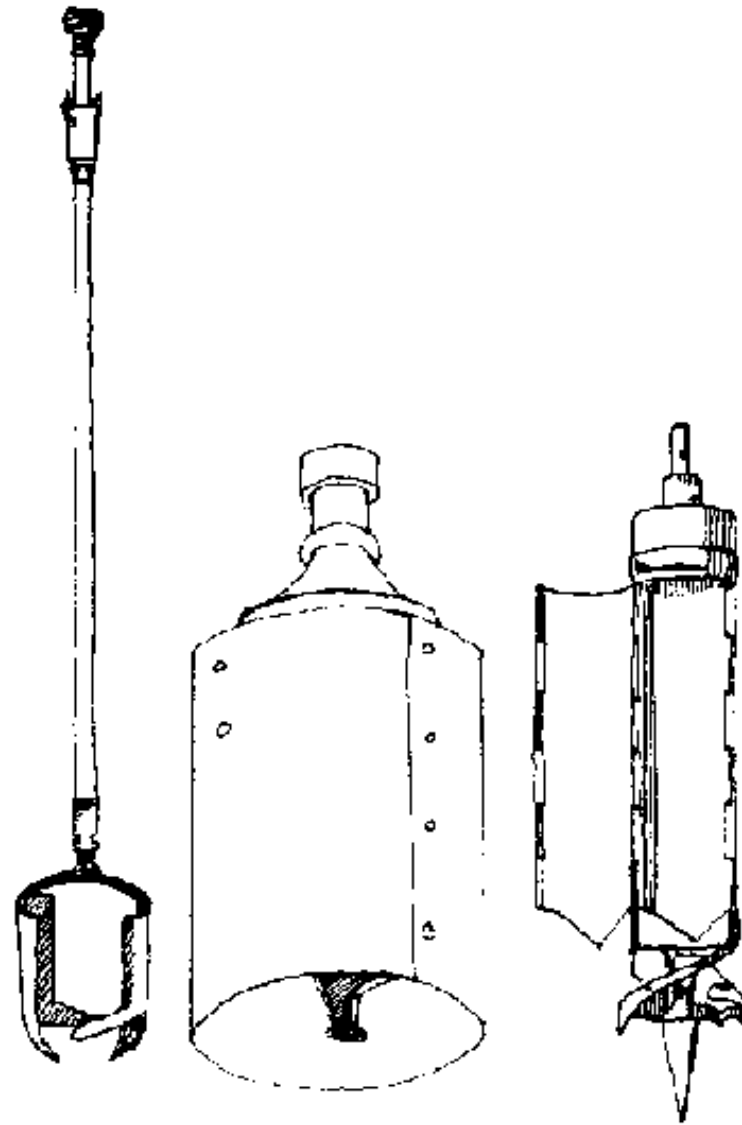
FIG. 12-2. BUCKET AUGERS
