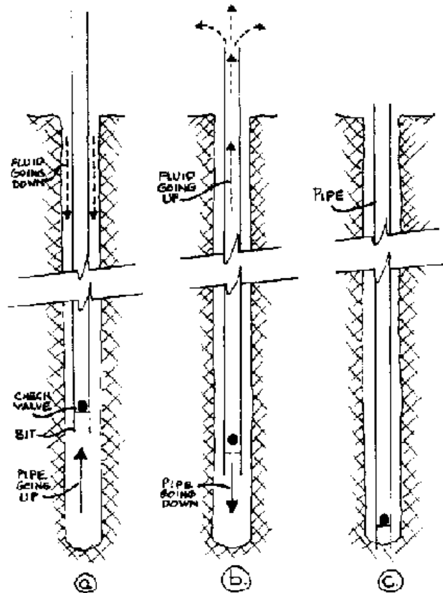
FIG. 13-1. SLUDGER DETAIL
