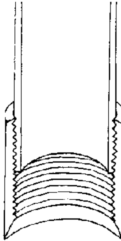
FIG. 11-9. SHARPENED COUPLING
