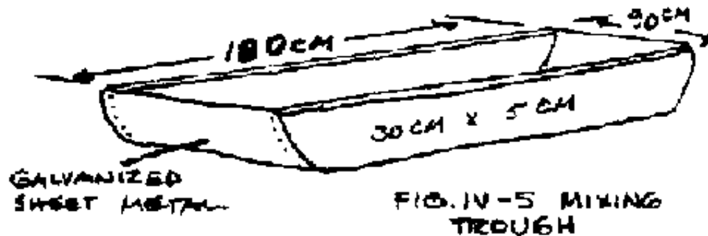
FIG. IV-5. MIXING TROUGH
