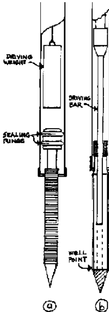
FIG. 14-7. STEEL DRIVING BAR ARRANGEMENT
