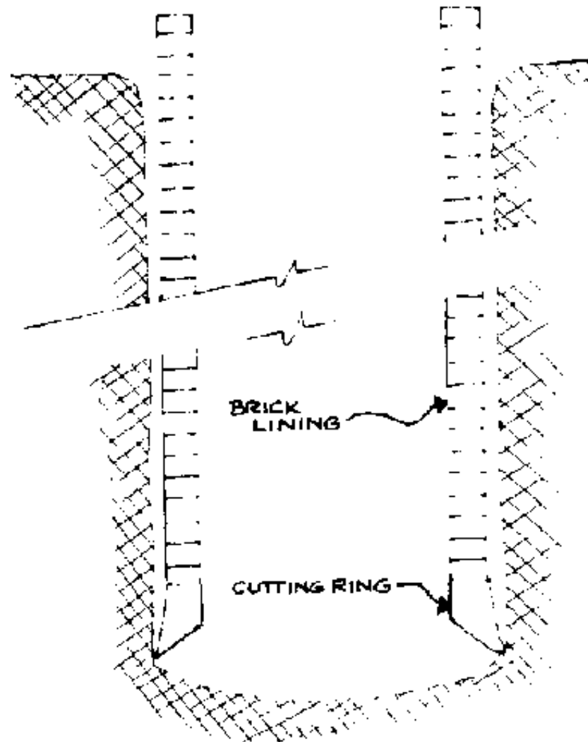
FIG. 8-14. BRICK LINING SUCK ON A CUTTING RING
