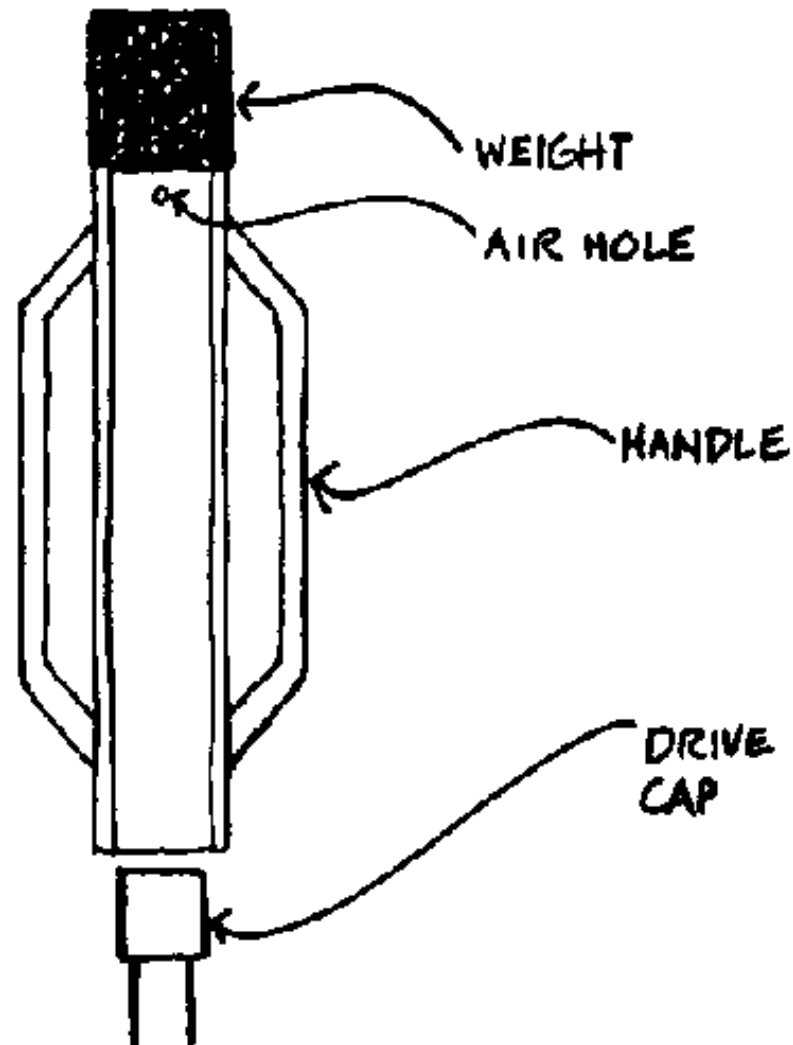
FIG. 14-6. WEIGHTED DRIVER
