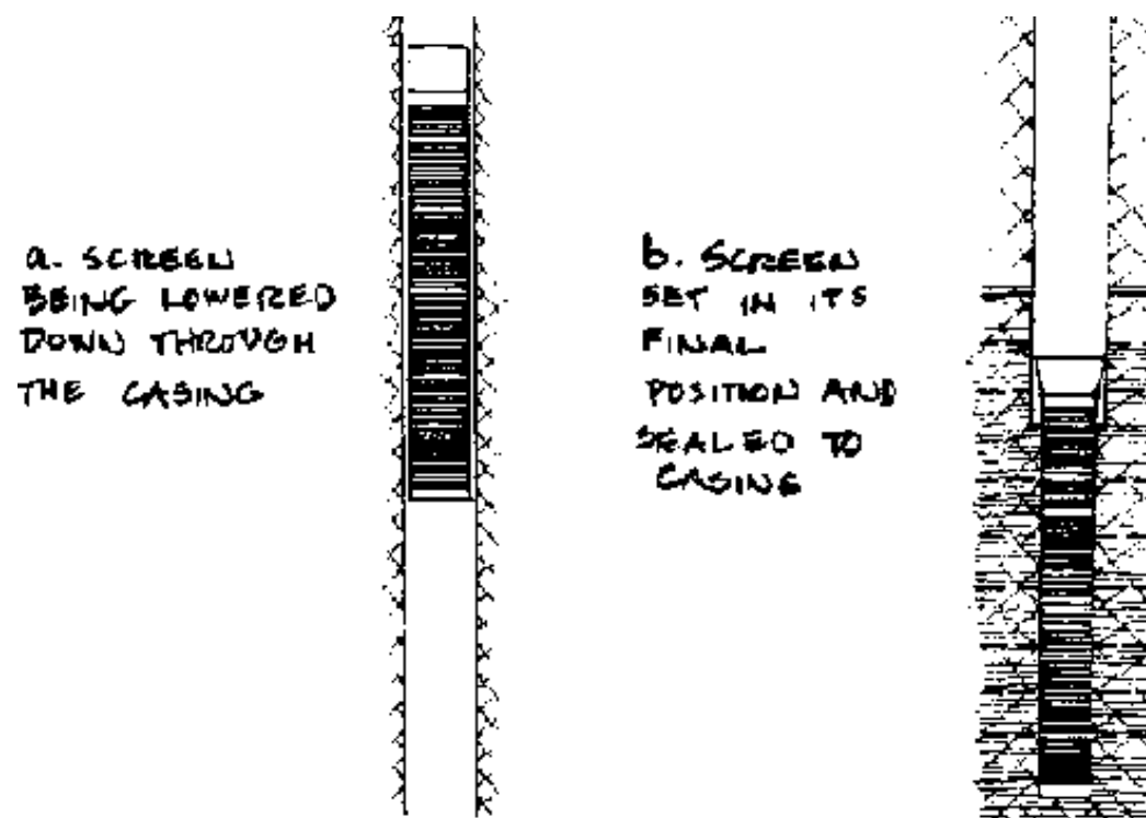
FIG. 15-6. TELESCOPING SCREEN
