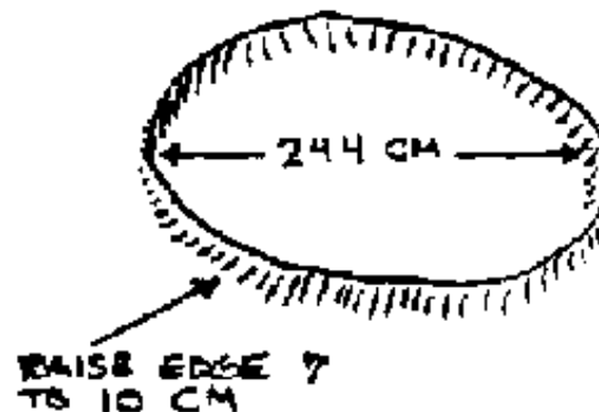
FIG. IV-6. MIXING PLATFORM
