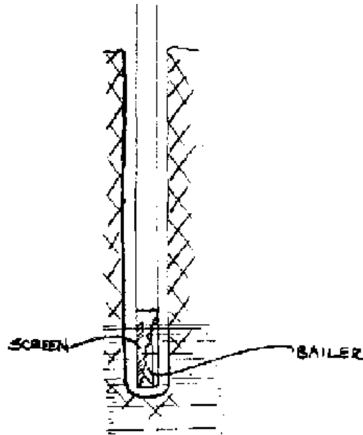
FIG. 15-8. SCREEN AND CASING BAILED DOWN
