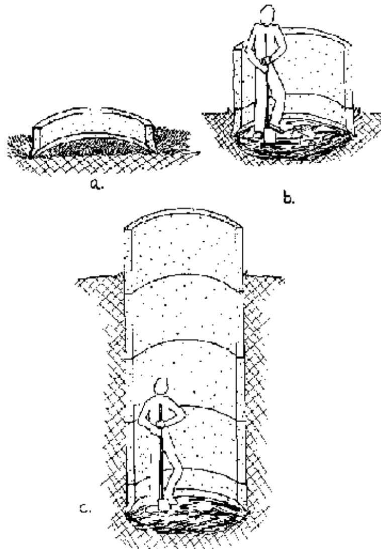
FIG. 8-10. SINKING LINING RINGS
