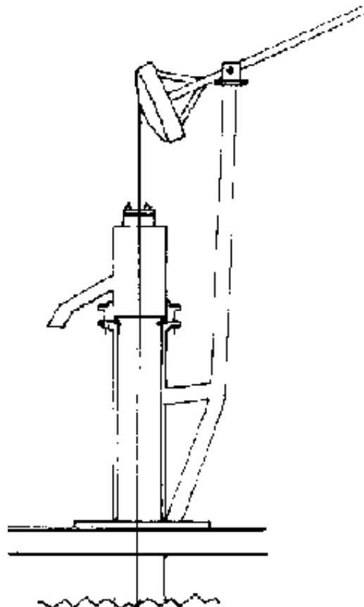
FIG. VII-8. LOCALLY MADE VARIATION OF JALNA PUMP
