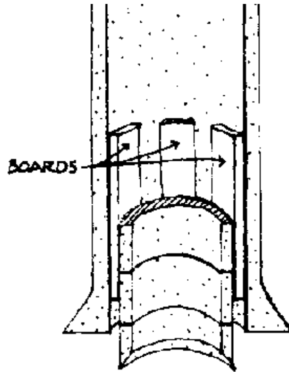
FIG. 9-6. BOARDS USED TO GUIDE SINKING RINGS
