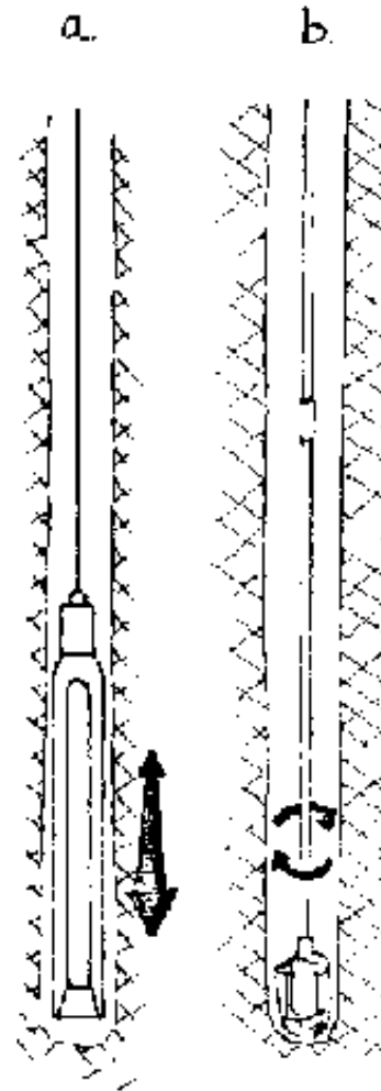
FIG. 10-2. DRILLING MOTIONS
