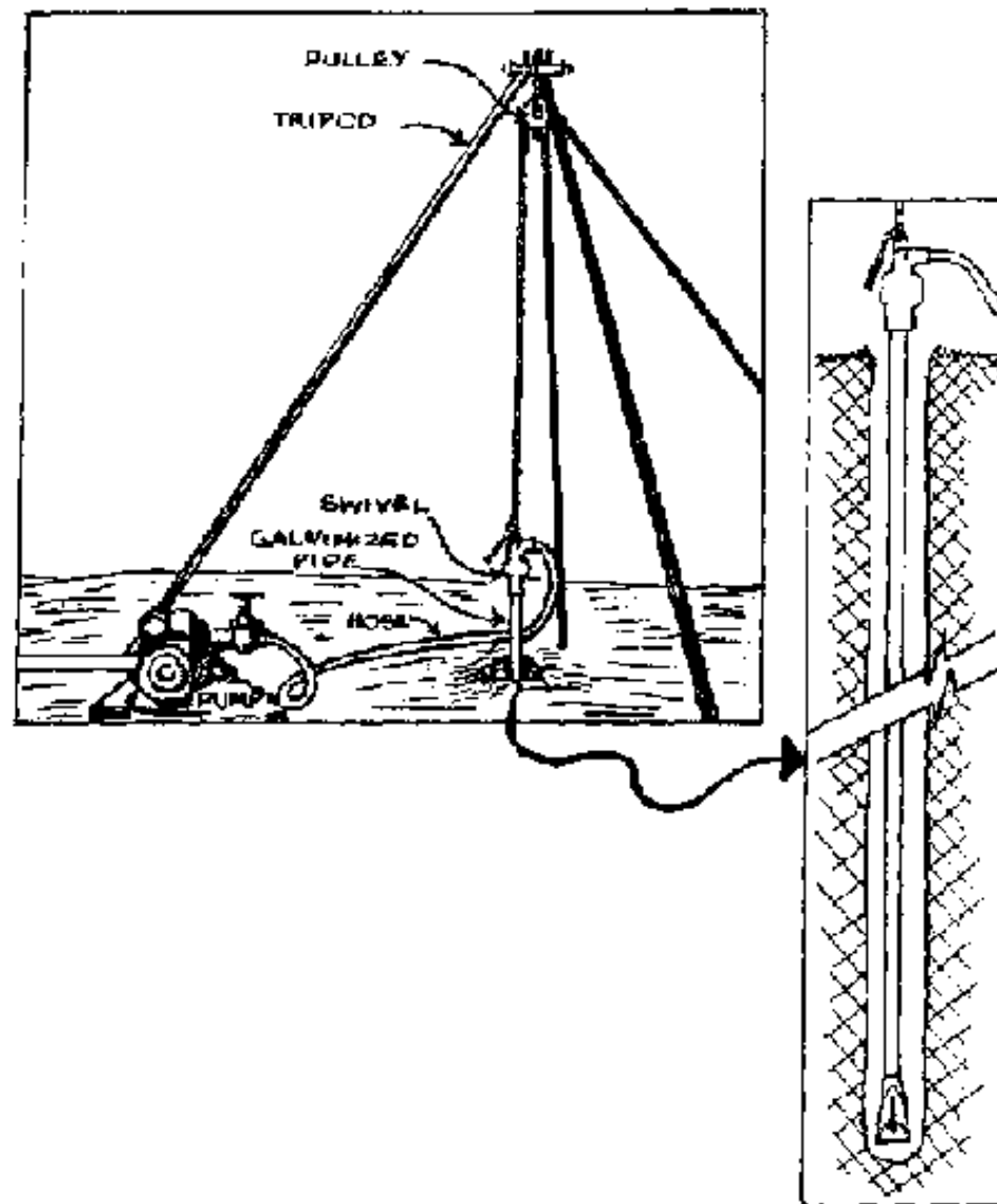
FIG. 11-8. JETTED WELL
