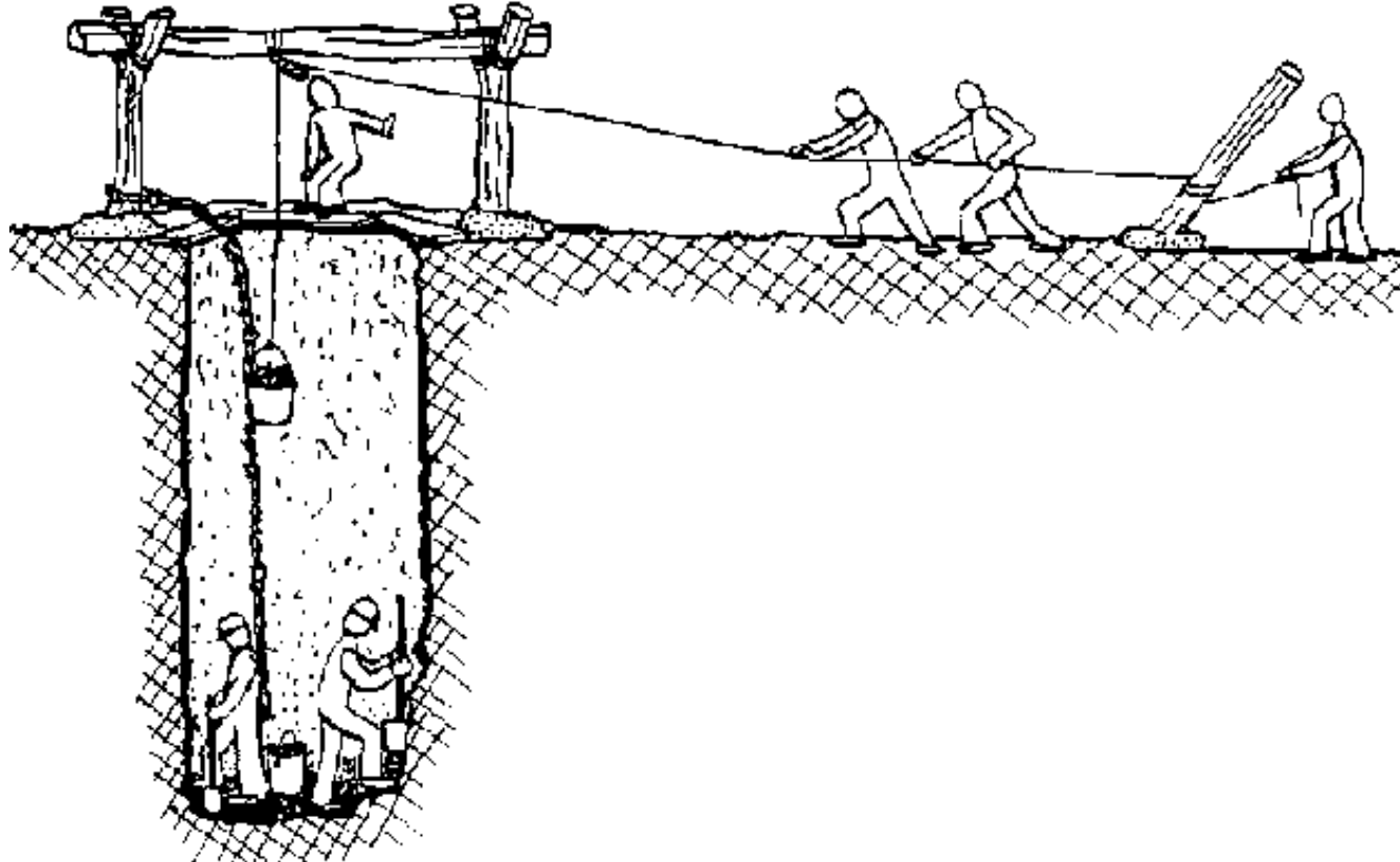
FIG. 5-1. RAISING AND LOWERING OPERATION
