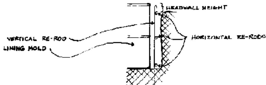
FIG. 8-3. PLACEMENT OF RE-ROD AND FORM IN HOLE
