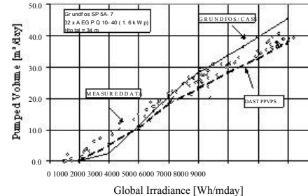
Figure 3: Comparison of measured data and computer design results using DASTPVPS and Grundfos-CASS software.
