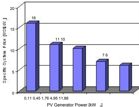
Figure 4: Specific PVP system prices (ex-works) without water tank, fence and surface piping (Source: Siemens Solar)
