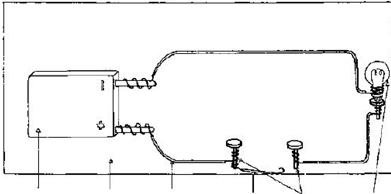
battery wood or cardboard conduction switch drawing-pins bulb
