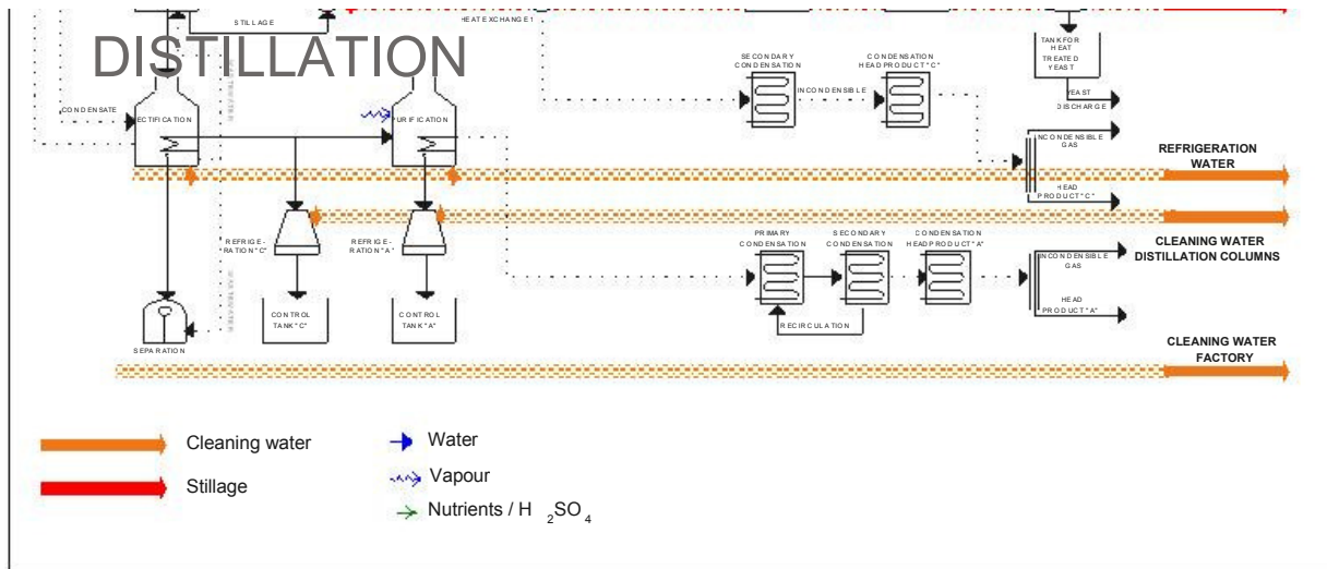
Fig. 2: Alcohol production and wastewater streams (Source: TBW, [3])
