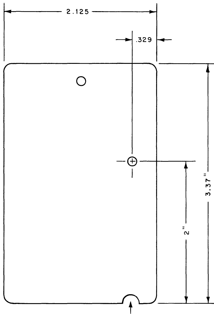
LOCATOR NOTCH OVERALL DIMENSIONS
