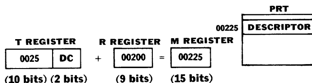
Figure 2-11. Referencing a Descriptor
