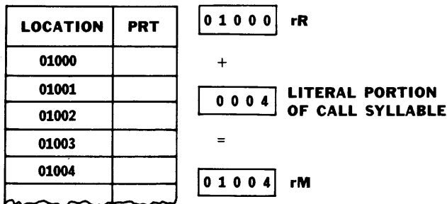
Figure 3-3. Indexing the PRT
