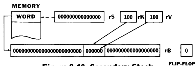
Figure 2-18. Secondary Stack and Destination Registers
