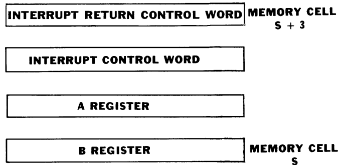
Figure 2-22. Resulting Stack In Memory—Interrupt Control
