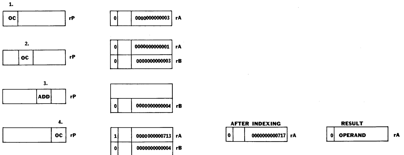
Figure 3-9. Variable Indexing
