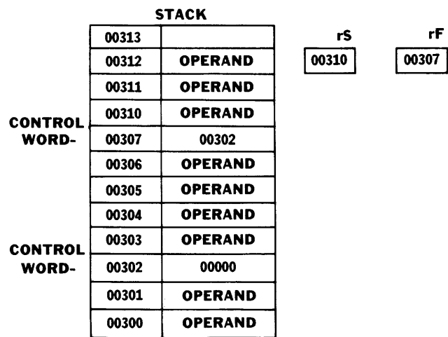
Figure 2-19. Subroutine Nesting Control
