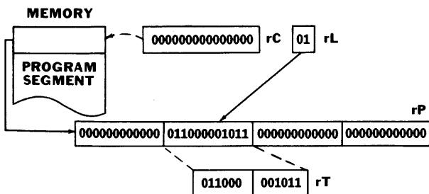
Figure 2-16. Program Registers
