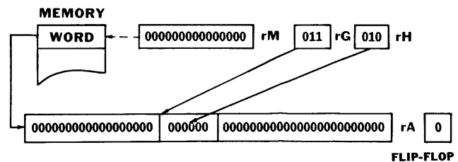
Figure 2-17. Primary Stack and Source Registers
