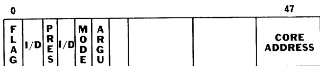
Figure 2-9. Program Descriptor
