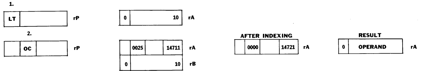
Figure 3-8. Constant Indexing
