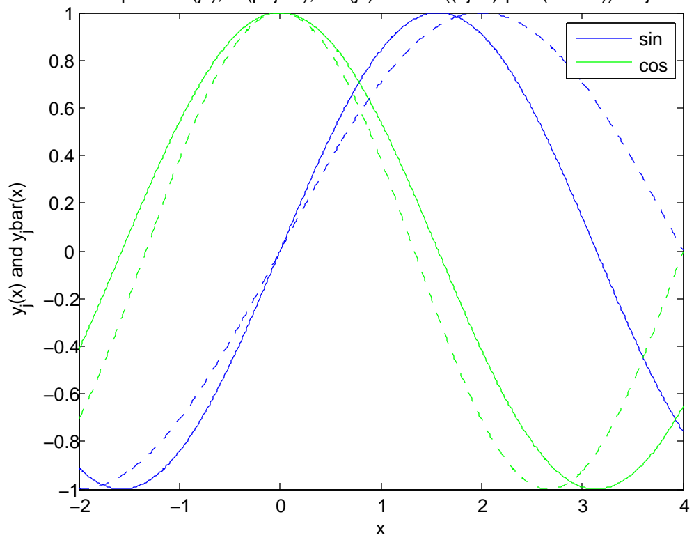
Graph of \sin(jx) , \sin(\pi*jx/4) , \cos(jx) and \cos((2j+1)*\pi*x/(2*\beta)) for j=1
