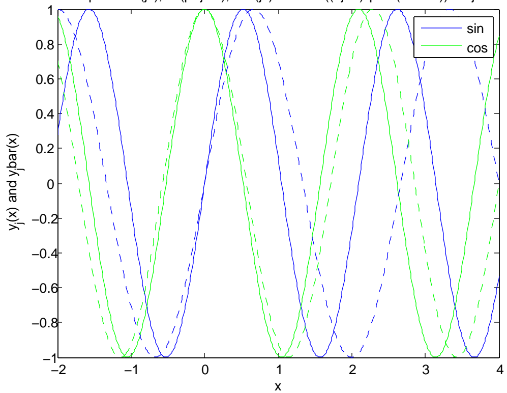
Graph of \sin(jx) , \sin(\pi*jx/4) , \cos(jx) and \cos((2j+1)*\pi*x/(2*\beta)) for j=3
