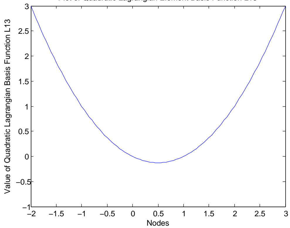
Plot of Quadratic Lagrangian Element Basis Function L13
