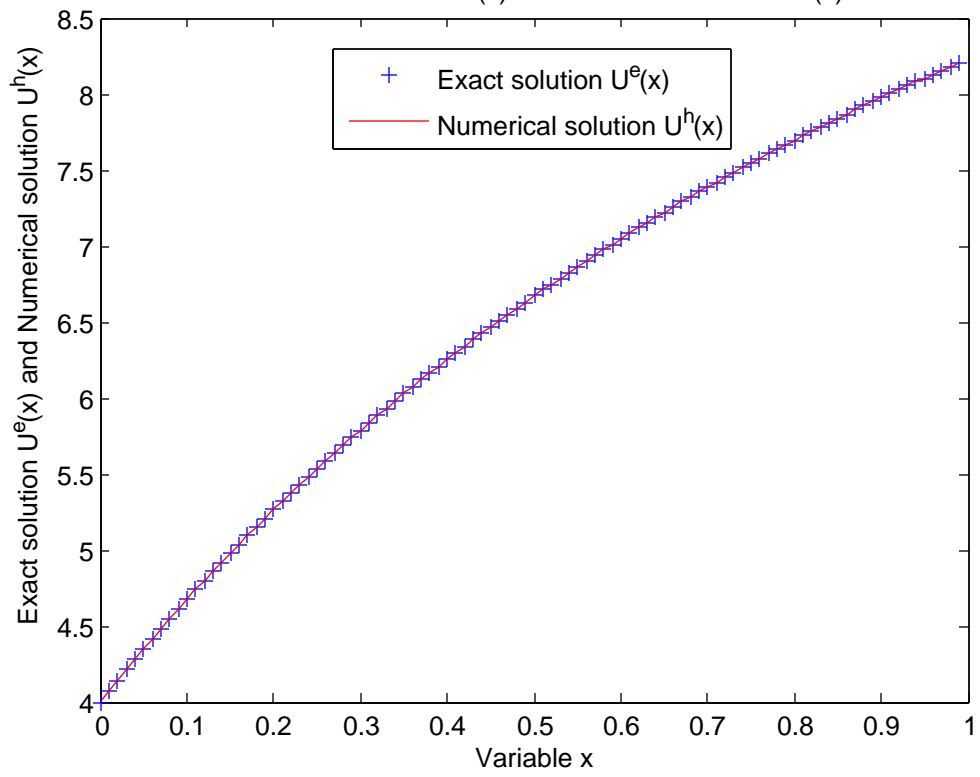
Exact solution U^e(x) Vs. Numerical solution U^h(x)
