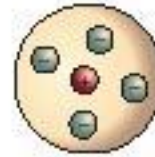
Rutherford's atom
