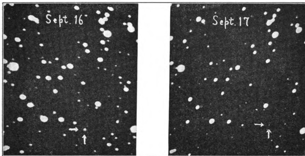
IN THESE PHOTOGRAPHS HALLEY'S COMET IS INDICATED BY THE ARROWS.
