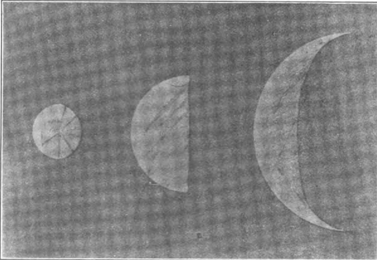
THE PLANET VENUS.
