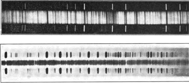
SPECTROGRAM OF JUPITER ABOVE AND OF VENUS BELOW, SHOWING IRON COMPARISON.
