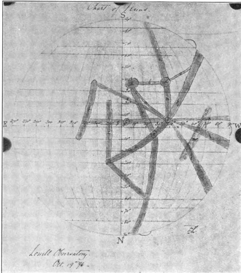
CHART OF THE PLANET VENUS.
