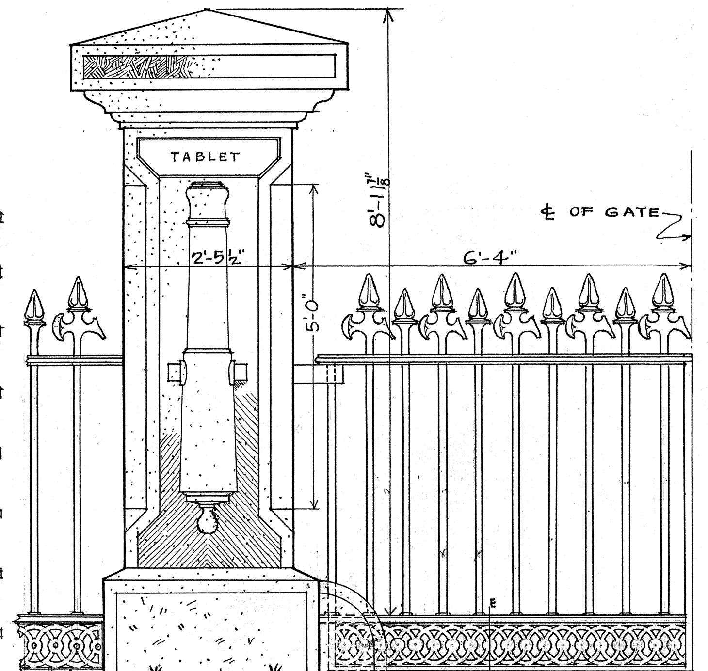
GATE AND GATE POST ELEVATION
