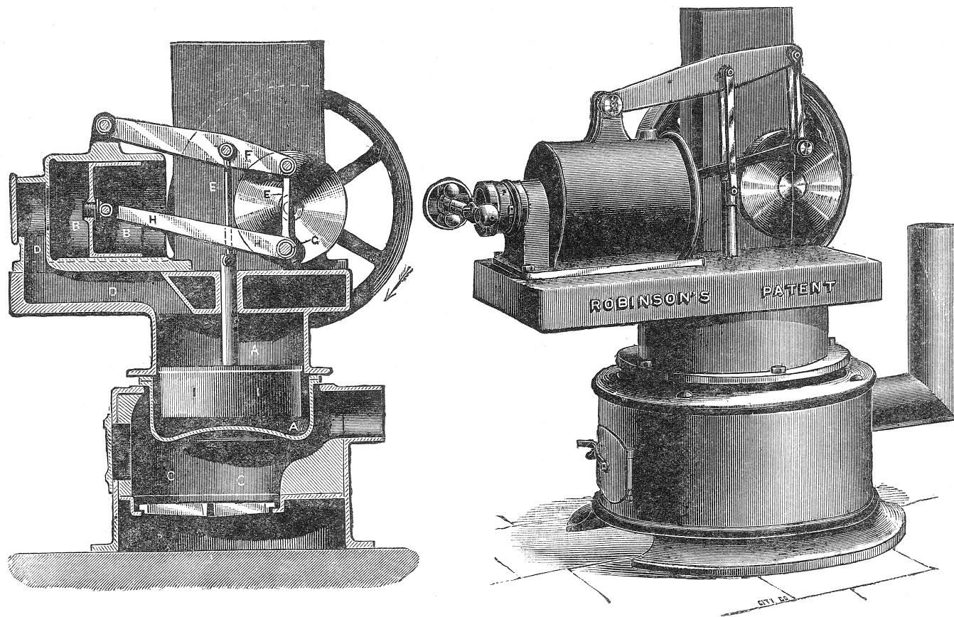
FIG. 47.—Robinson's Engine.
