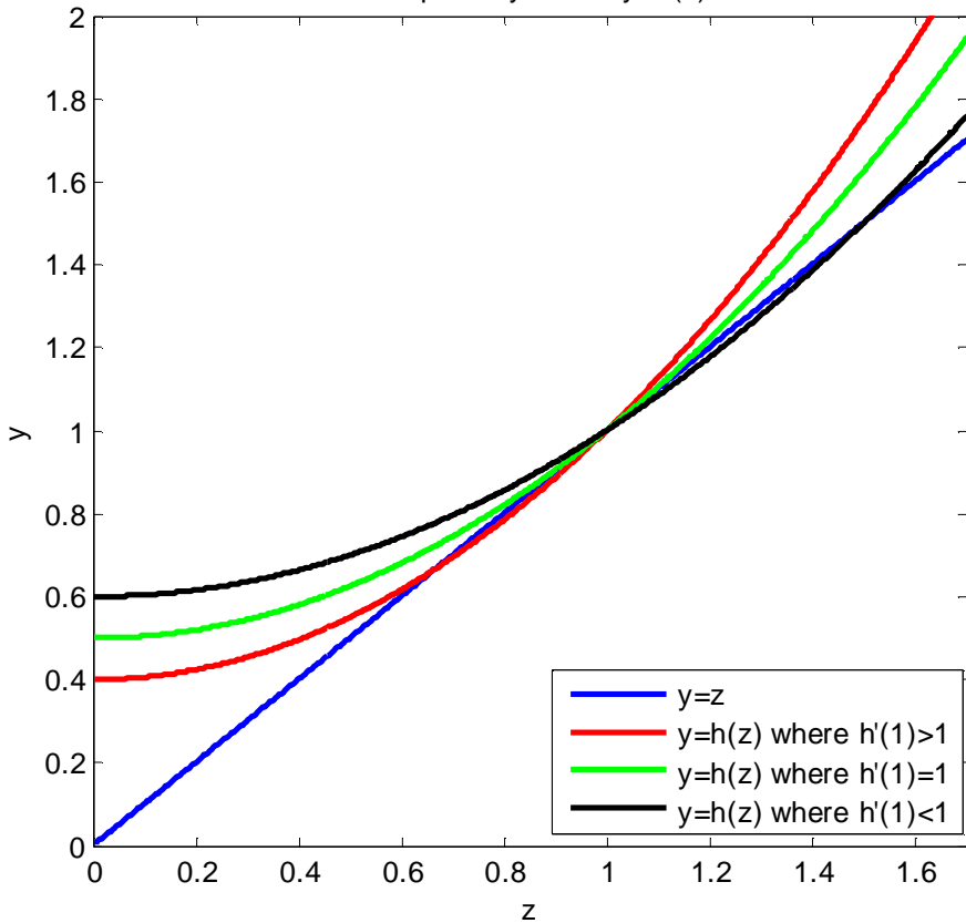
Graphs of y=z and y=h(z)
