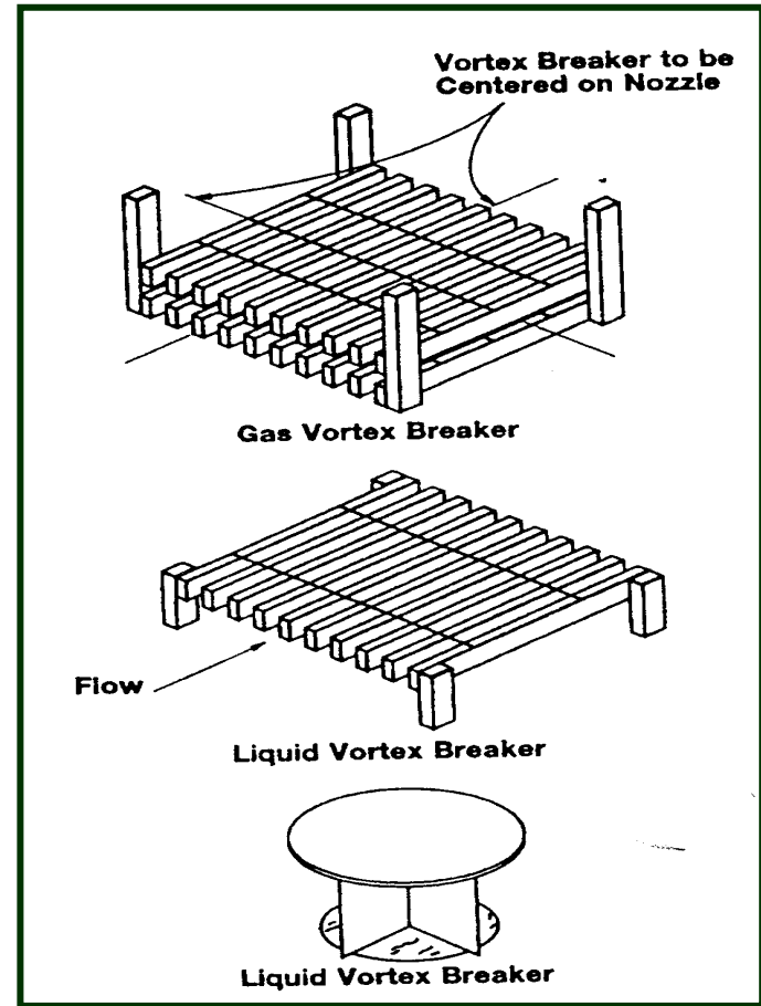
Liquid and Gas Vortex Breakers
