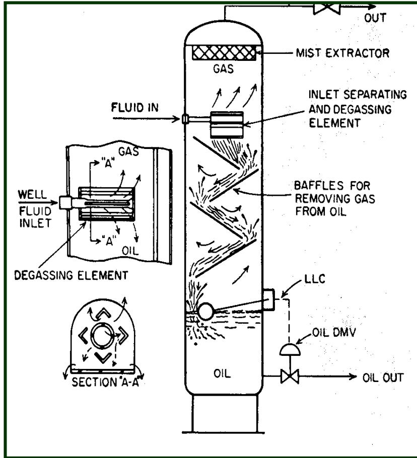
Vertical Separator for Foaming Crude Oil
