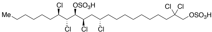
danicalipin A
