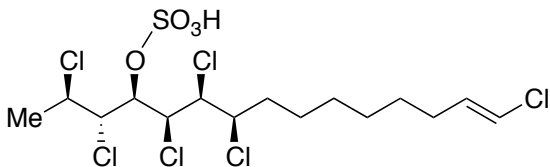
hexachlorosulfolipid
