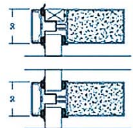
Snit F-F
