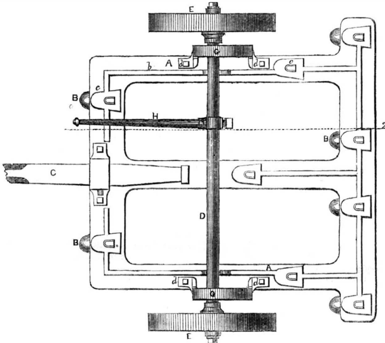
IMPROVED CULTIVATOR.—Figure 1.
