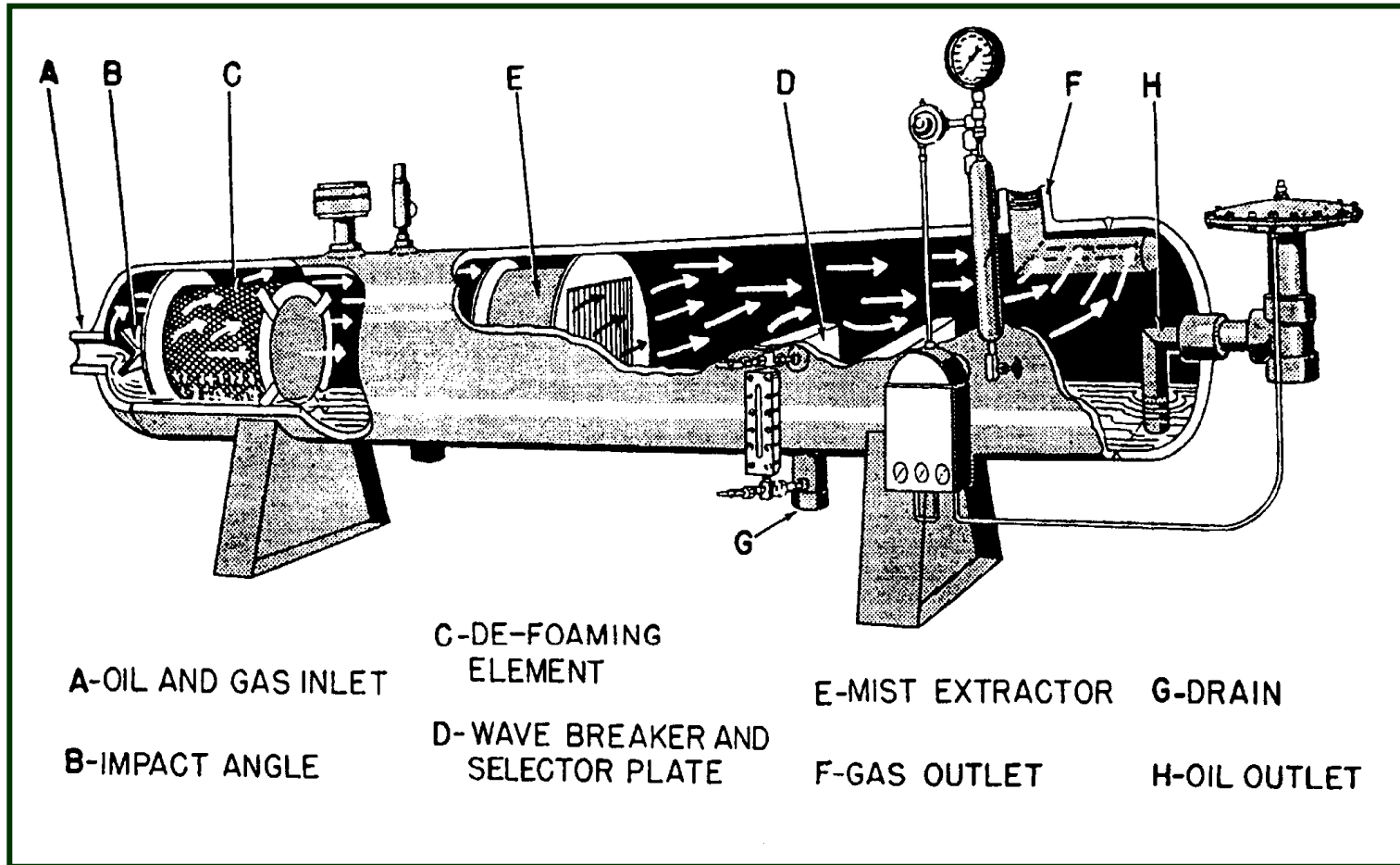
Typical Single-Tube Horizontal Separator
