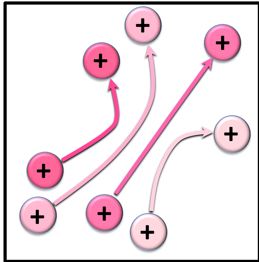
Liouvillian mechanics
