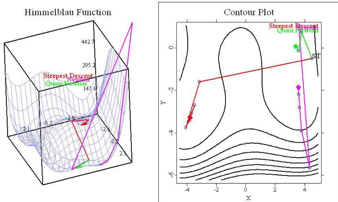
Figure 19: Figure 2: Even all methods find different solutions.
