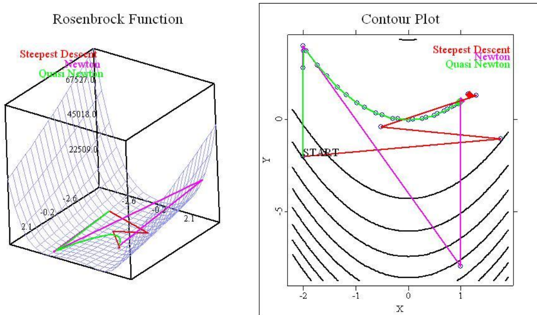
Figure 21: Figure 2: Overshooting of the Newtonian Method due to the fixed stepsize.
