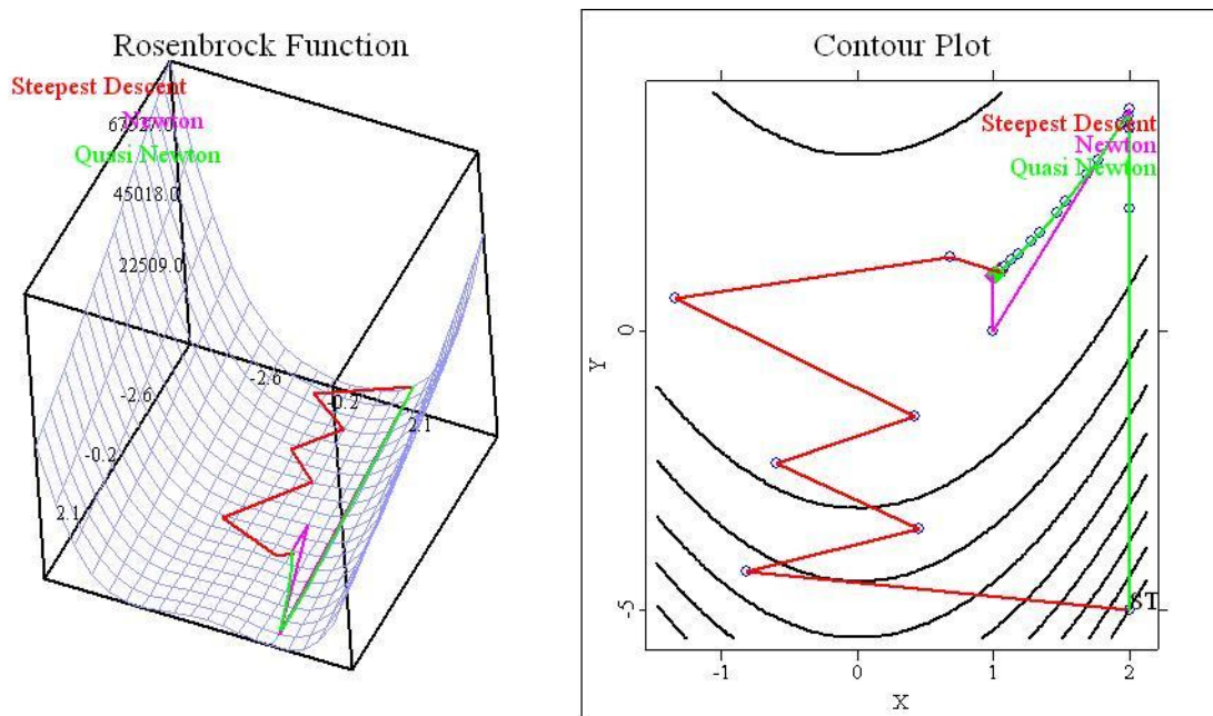
Figure 20: Figure 3: All methods find the same solution, but the Method of Steepest Descent fluctuates heavily.
