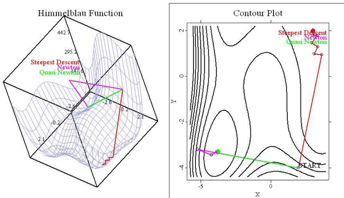
Figure 18: Figure 1: The two Newton Methods converge to the same, the Method of Steepest Descent to a different minimum.
