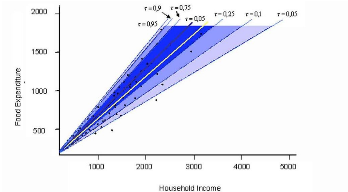
Abb. 23: Figure 2: Engels Curve, with the median highlighted in dark blue and the mean in yellow
