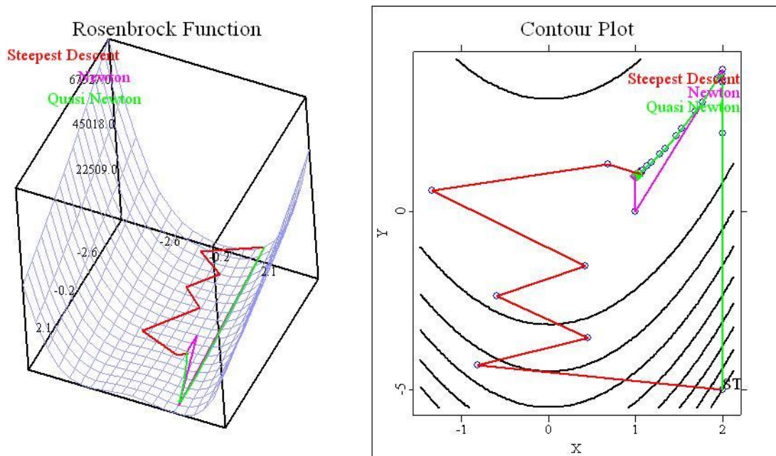
Abb. 20: Figure 3: All methods find the same solution, but the Method of Steepest Descent fluctuates heavily.
