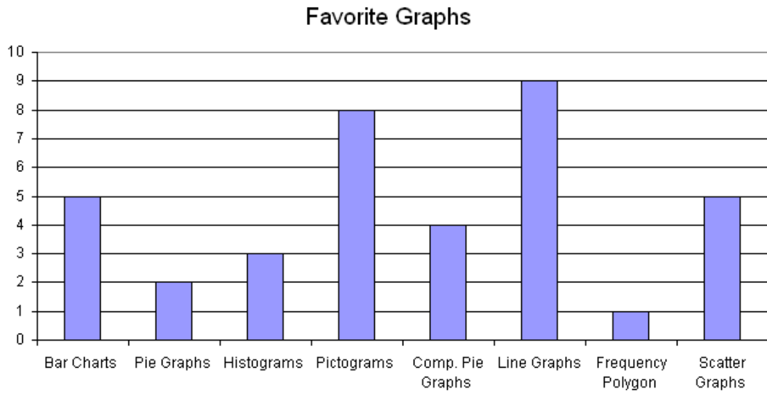
Abb. 2: Vertical Bar Chart Example
