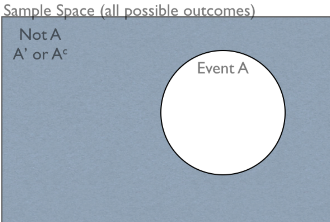
Abb. 15: Complement of an Event
