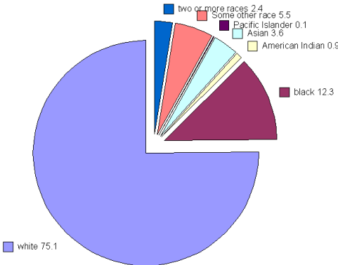
Abb. 8: A pie chart showing the racial make-up of the US in 2000.
