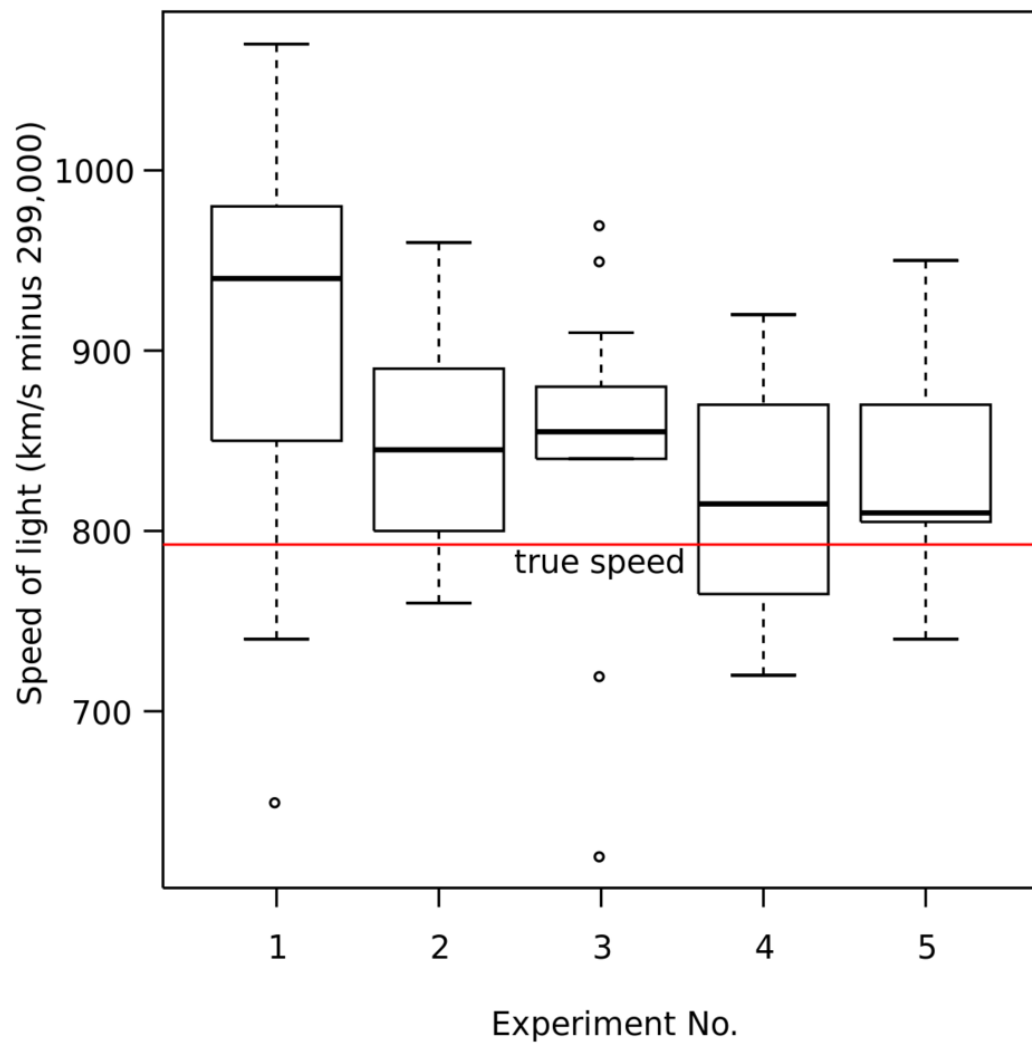
Abb. 7: Figure 1. Box plot of data from the Michelson-Morley Experiment
