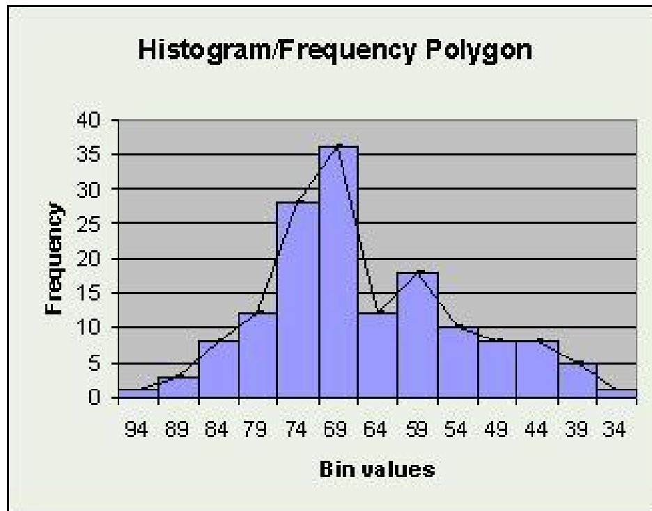
Abb. 12: This is a histogram with an overlaid frequency polygon.
