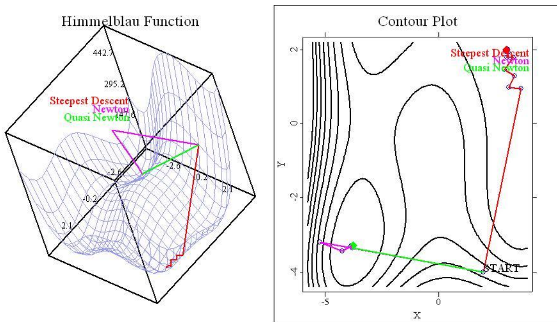
Abb. 18: Figure 1: The two Newton Methods converge to the same, the Method of Steepest Descent to a different minimum.
