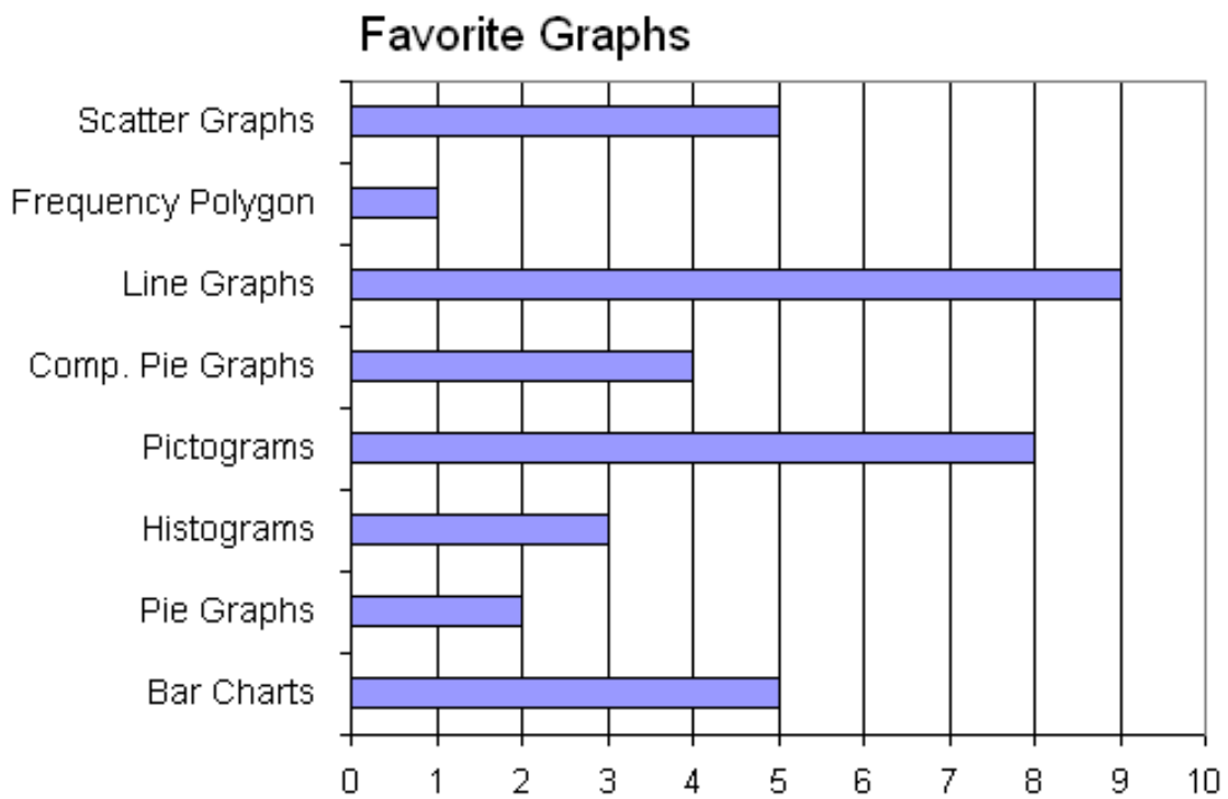
Abb. 3: Horizontal Bar Chart Example
