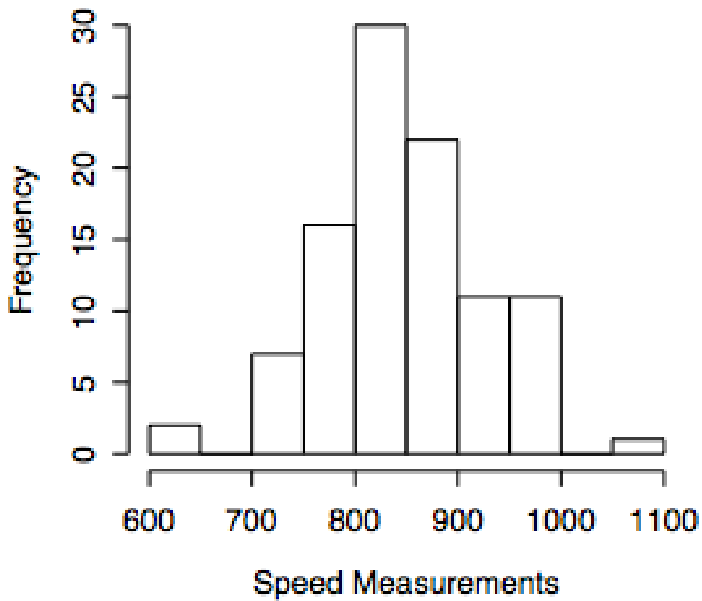
Michaelson-Morley Speed of Light Data
