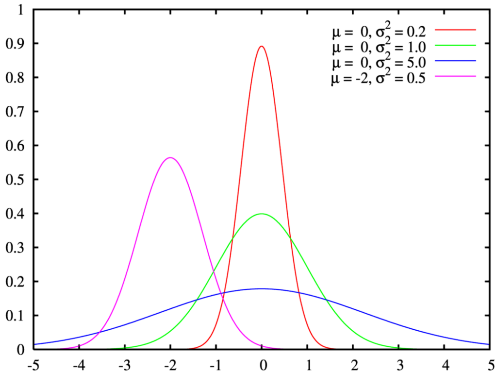
Abb. 1: Probability density function for the normal distribution. The green line is the standard normal distribution.
