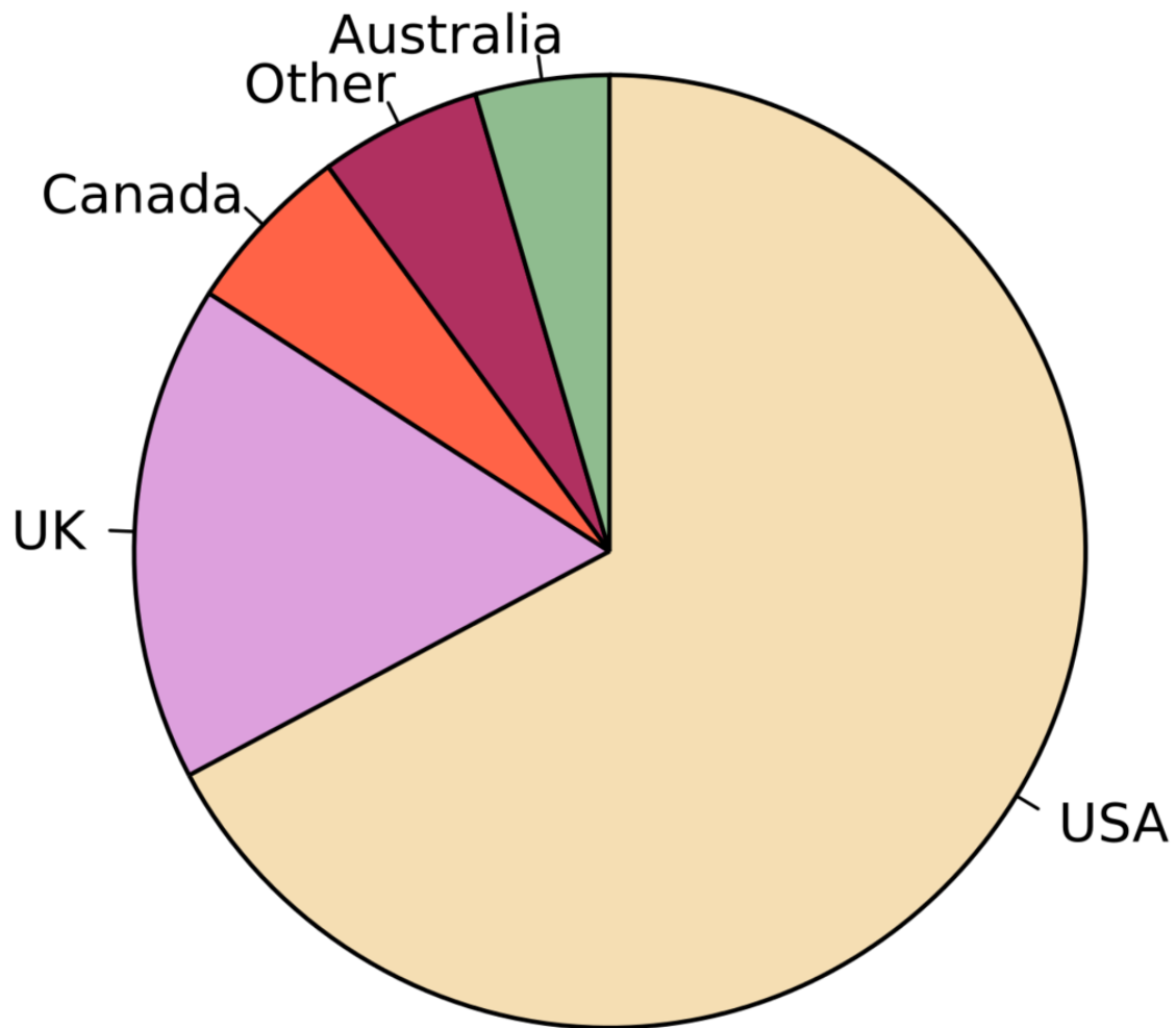
Abb. 9: Pie chart of populations of English language-speaking people
