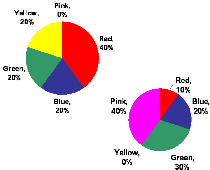
Abb. 10: A pie chart showing preference of colors by two groups.
