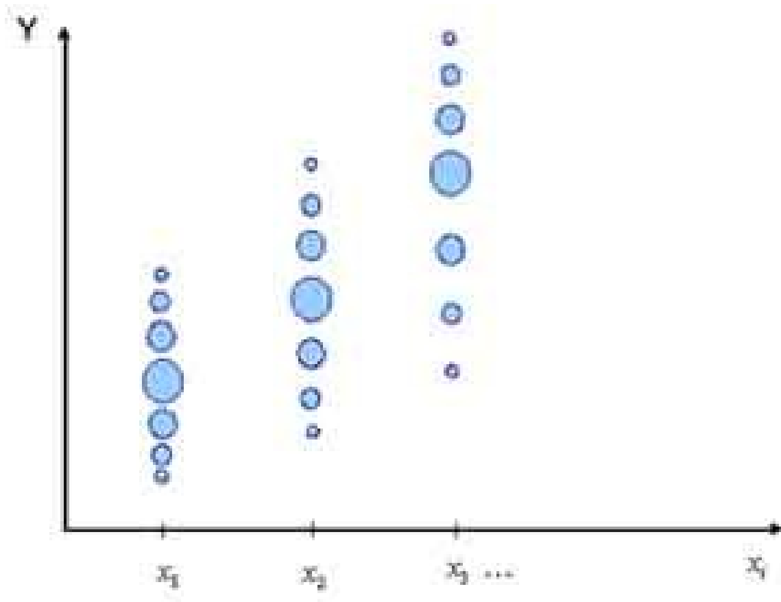
Abb. 22: Figure 1: Probabilities of occurrence for individual explanatory variables
