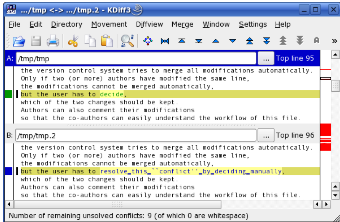
Figure 108: Figure 2: Reviewing modifications in KDiff3
