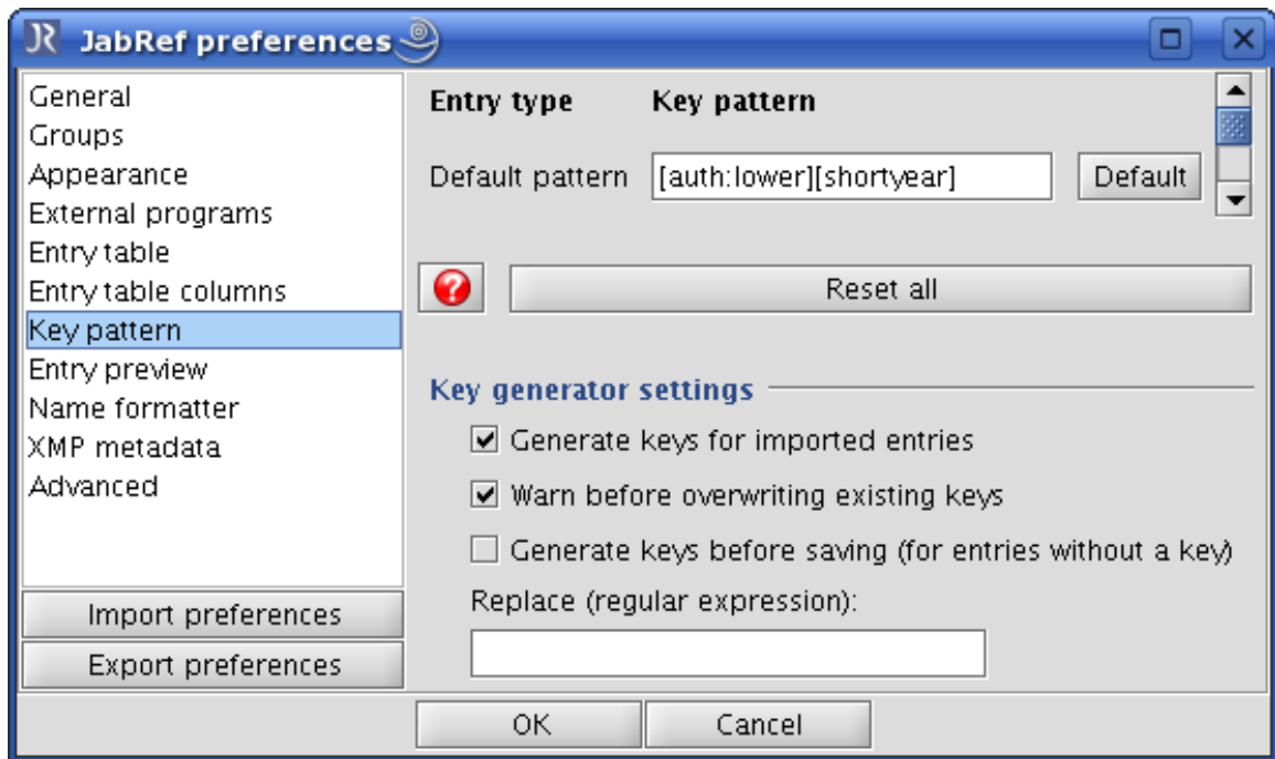
Figure 109: Figure 3: Specify default key pattern in JabRef
