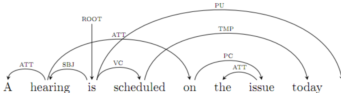
Figure 93: A dependency tree drawn with TikZ-dependency.
