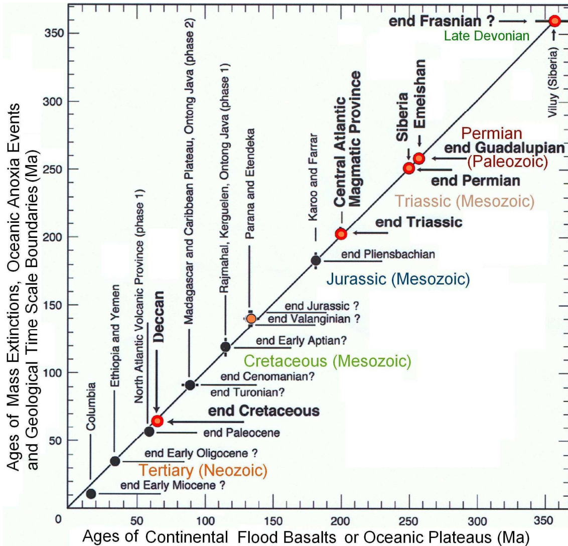
Fig. 7: Time-correlation of mass-extinctions and flood-basalt-events. Graphic: COURTILOT / RENNE: Comptes Rendus Geoscience 335(1) 2003.
