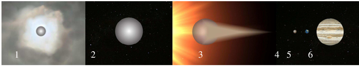
Fig. 8: Origin of planets as gas-giants [19].
