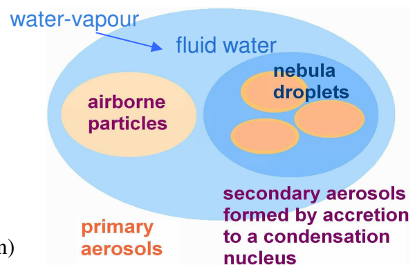
Fig. 2: Secondary aerosols as starting basis for a hydrous accretion
