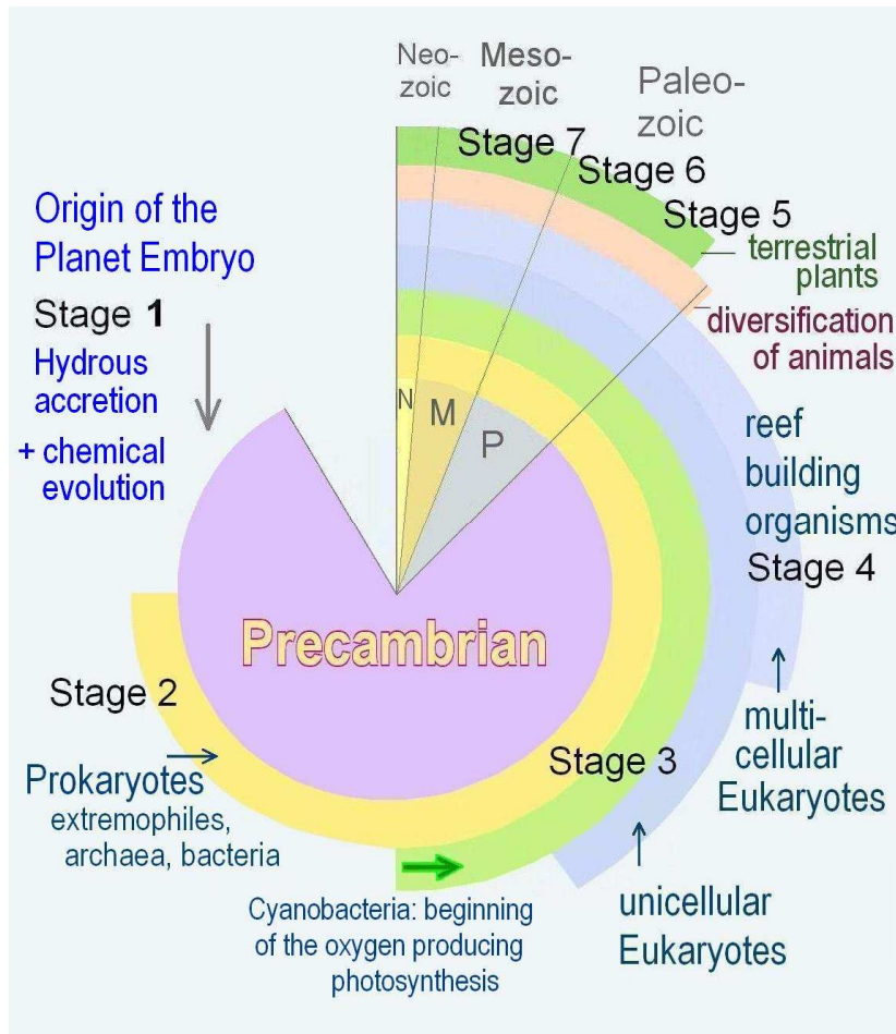
Fig. 3a: Timescale of early evolution and biodiversification.
