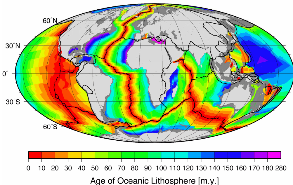
Fig. 36: Spreading-zones produce oceanic crust symmetrically to both sides. The area symmetrically corresponding to the round Jurassic crust submerged under America. The oldest ocean-floor is under the Mediterranean because the moon came from east (cp. Fig. 12). In Paleozoic moon caused a spreading-zone in the Tethys dividing Greece and Italy from Africa. Since Jurassic the ring of spreading-zones on the southern hemisphere pushes Africa towards Eurasia, so that the Mediterranean became a subduction-zone.
