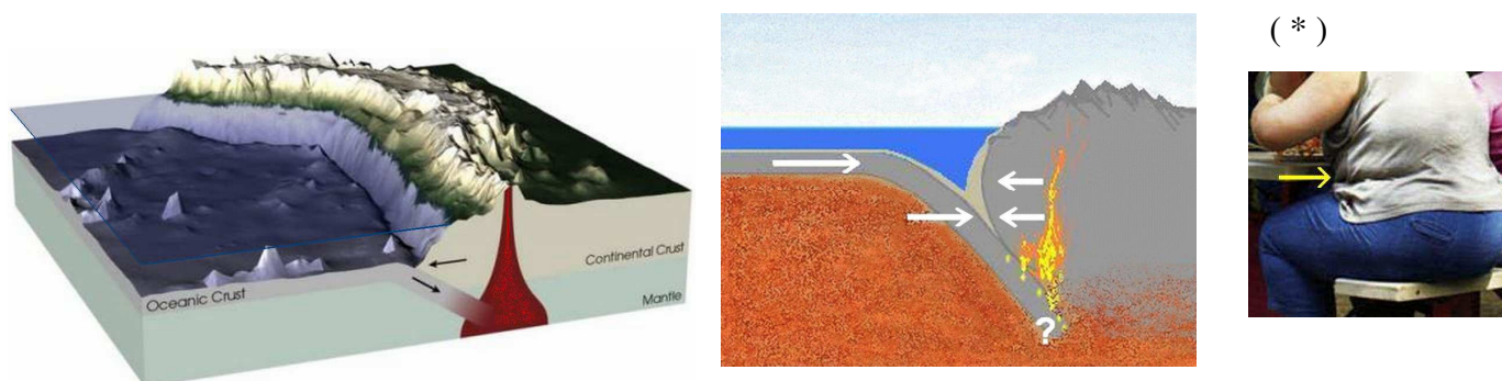
Fig. 33: Paintings of subduction-zones, each one with another problem. On the left the continental-crust was put proportionally like an iceberg in the sea-water instead of in the upper mantle. This was done because the density of the upper mantle is so high, that the continental crust cannot be deeper. The same applies for the oceanic crust. On the right the continental crust is deeper, but the oceanic crust cannot merge so deep without melting and being transformed chemically. (*) If subduction could prevent an increase of volume, that would be a relief for people suffering from overweight.)
