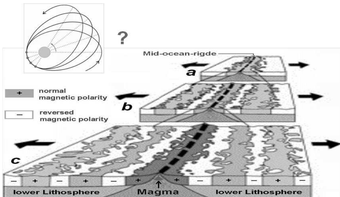
Fig. 37: Symmetrical ocean-floor-basalts show repeated changes of magnetic polarity.
