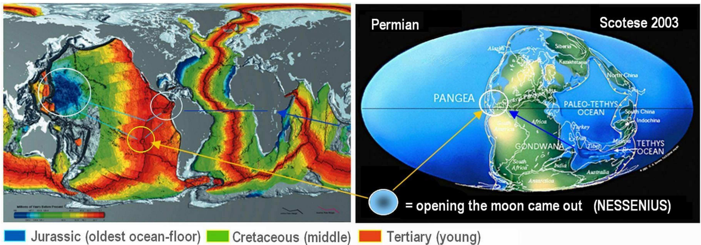
Fig. 9: Ages of origin of the oceanic crust. Fig. 10: Emerging of the moon in Permian.
