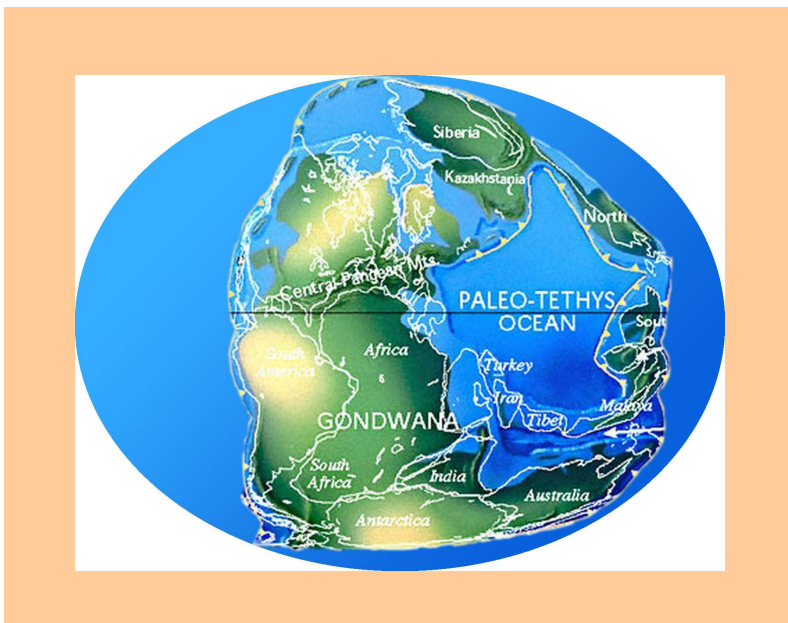
Fig. 6a: Paleomap Scotese (2003): Permian: High global temperature (cp. Fig. 3b).
