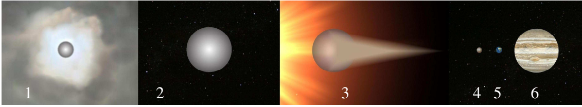
Fig. 8: Origin of planets as gas-giant of Jupiter-size as second stage [19].
