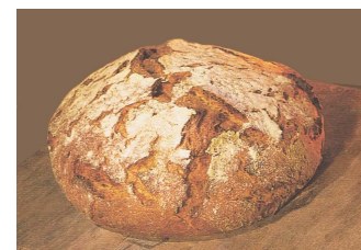
Fig. 6b: Interaction of exogenic and endogenic factors can be easily seen on the example: a loaf of bread being bake, contracting on the outside, expanding from inside, opening a „mid-ocean-ridge“.
