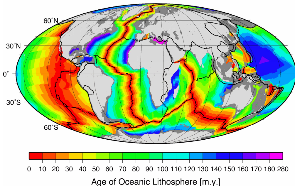
Fig. 35: Spreading-zones produce oceanic crust symmetrically to both sides. The area symmetrically corresponding to the round Jurassic crust submerged under America. The oldest ocean-floor is under the Mediterranean because the moon came from east (cp. Fig. 11). In Paleozoic moon caused a spreading-zone in the Tethys dividing Greece and Italy from Africa. Since Jurassic the ring of spreading-zones on the southern hemisphere pushes Africa towards Eurasia, so that the Mediterranean became a subduction-zone.
