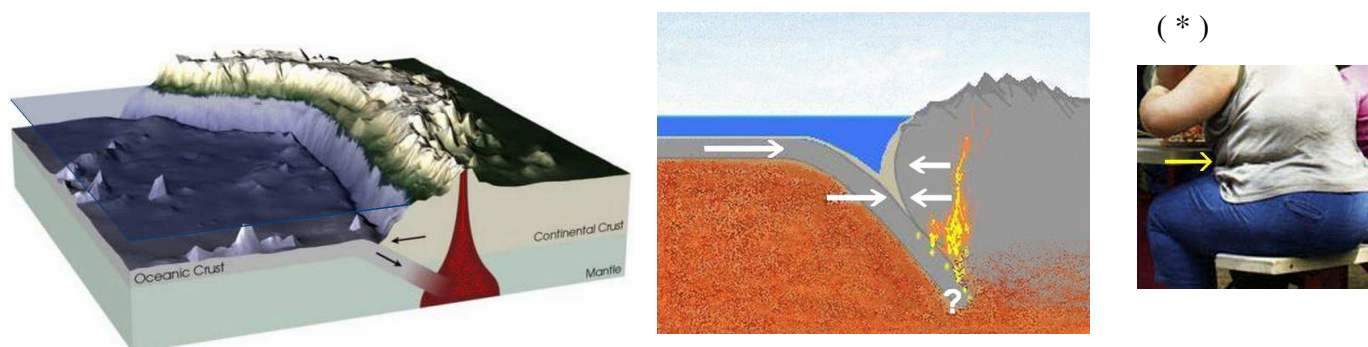
Fig. 32: Paintings of subduction-zones, each one with another problem. On the left the continental-crust was put proportionally like an iceberg in the sea-water instead of in the upper mantle. This was done because the density of the upper mantle is so high, that the continental crust cannot be deeper. The same applies for the oceanic crust. On the right the continental crust is deeper, but the oceanic crust cannot merge so deep without melting and being transformed chemically. (* If subduction could prevent an increase of volume, that would be a relief for people suffering from overweight.)
