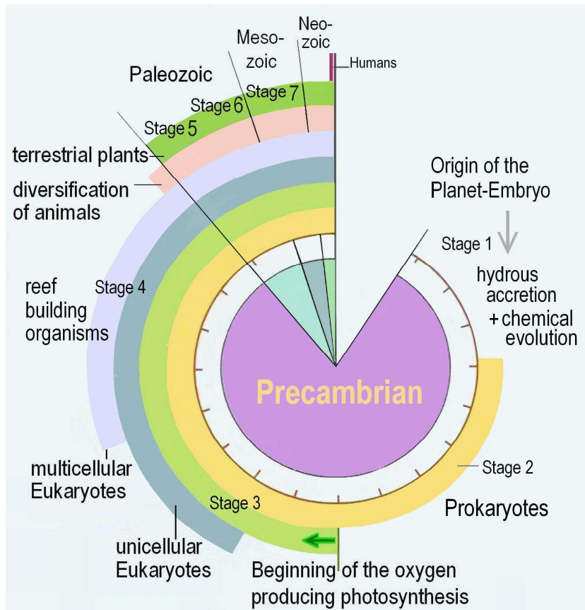
Fig. 3a: Timescale of early evolution and diversification.
