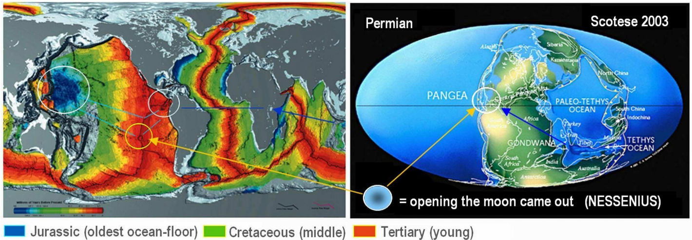
Fig. 8: Ages of origin of the oceanic crust. Fig. 9: Emerging of the moon in Permian.
