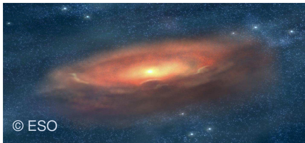
Fig. 1a: Protoplanetary disc (artist's impression)
