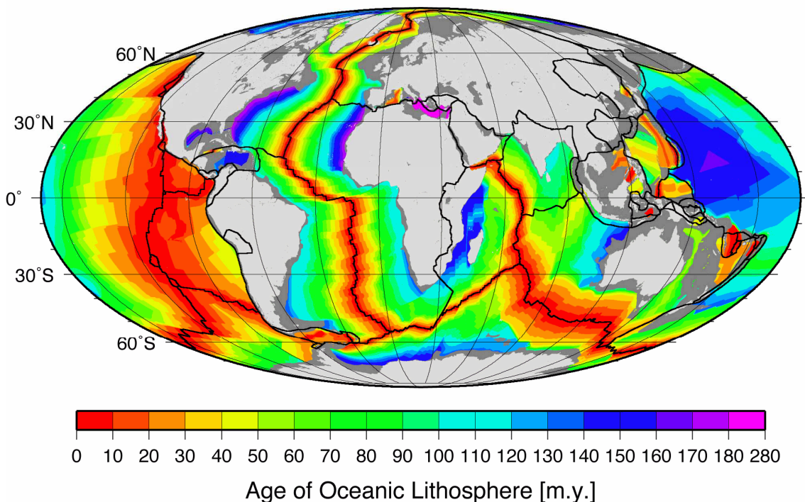
Fig. 35: Spreading zones produce oceanic crust symmetrically to both sides.
