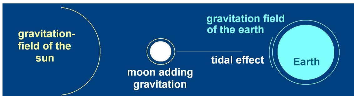
Fig. 34: Tidal effect of the moon.
