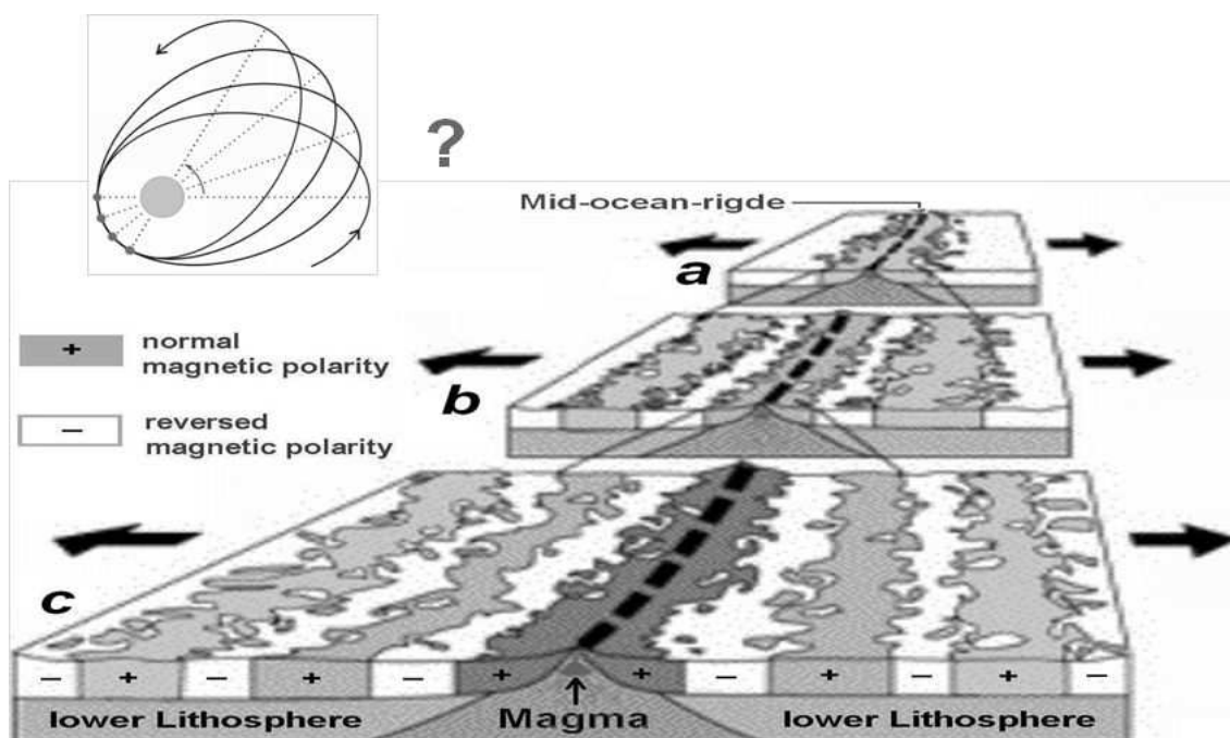
Fig. 35: Symmetrical ocean-floor-basalts show repeated changes of magnetic polarity.
