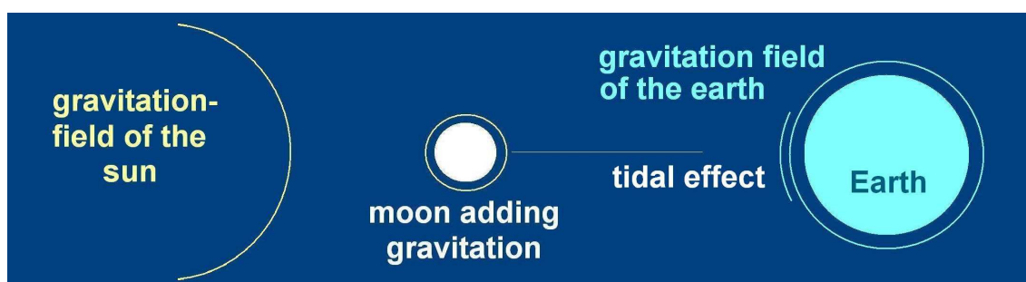
Fig. 34: Tidal effect of the moon.
