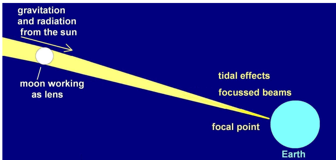
Fig. 33: Radiation being focussed by the moon working as lens.
