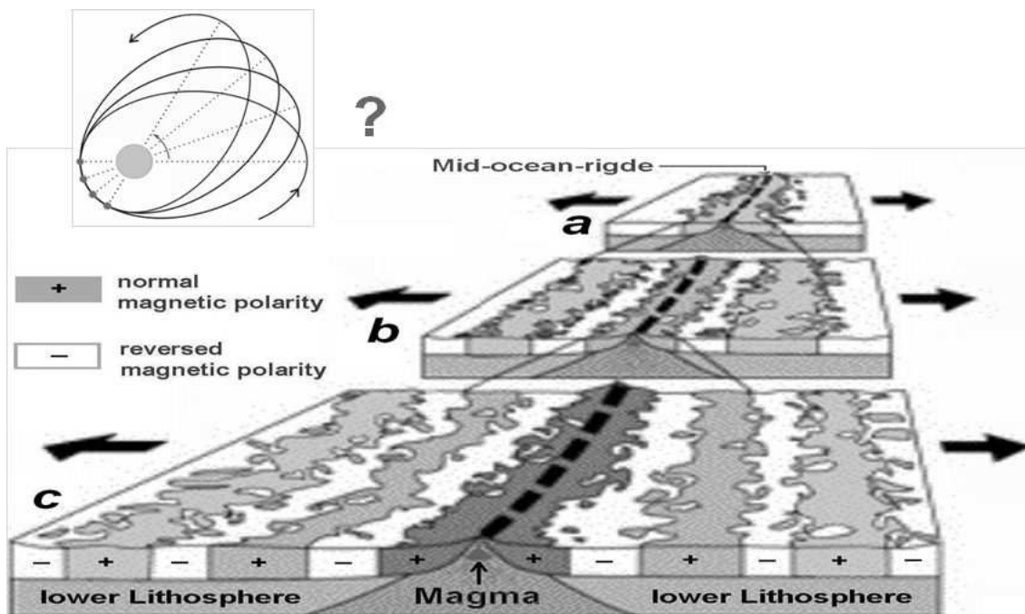
Fig. 34: Symmetrical ocean-floor-basalts show repeated changes of magnetic polarity.
