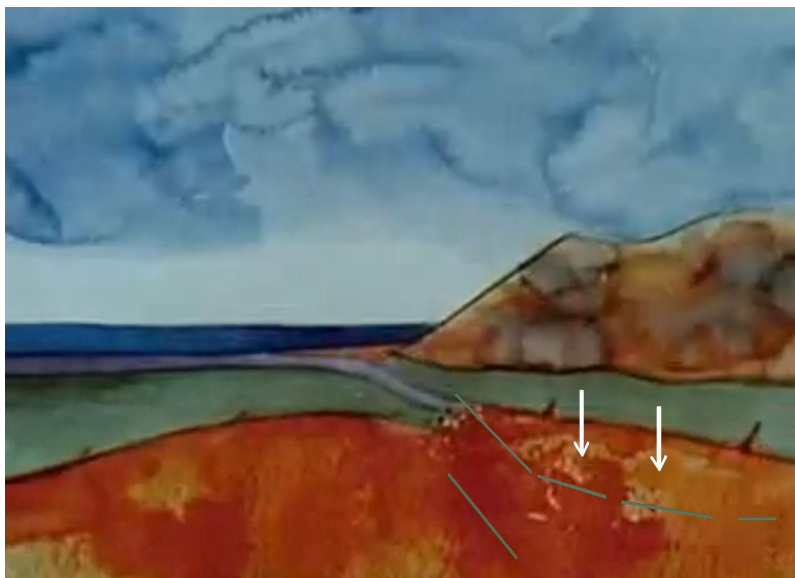
Fig. 32: Very beautiful but physically wrong painting of a subduction-zone.
