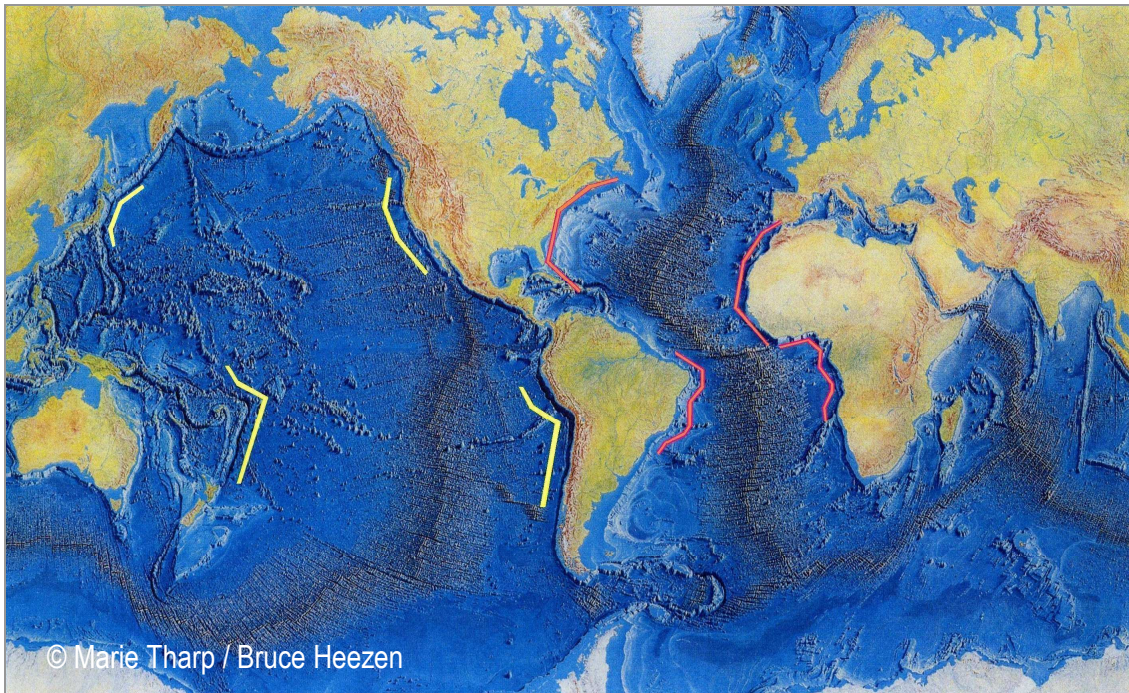
Fig. 10: World Ocean Floors in the Holocene, the latest time of the Neozoic. Before Permian the coast-lines (red and yellow) were located together as one not yet hardened but cohesive earth-surface. Bruce Heezen himself suggested earth-expansion.
