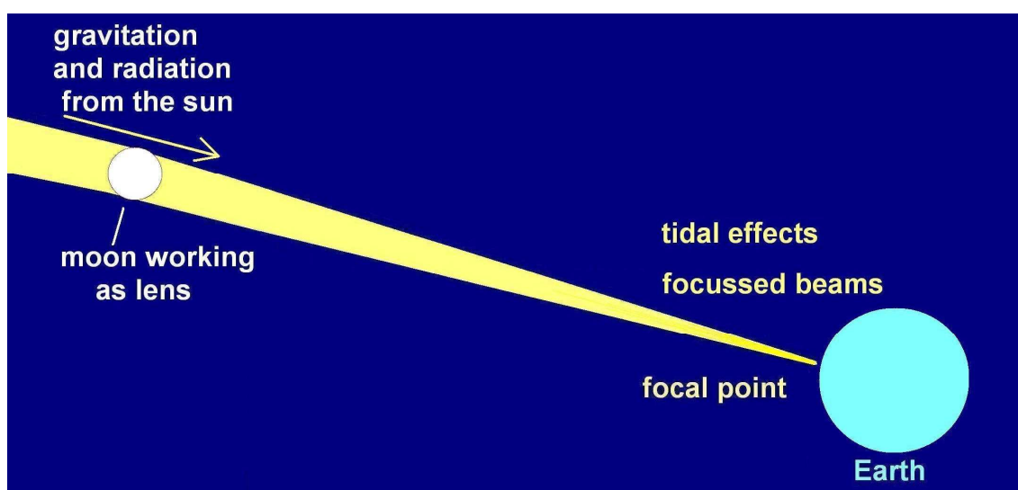
Fig. 32: Radiation being focussed by the moon working as lens.
