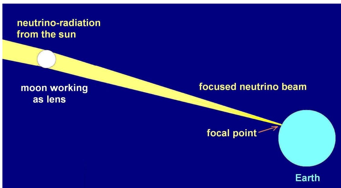
Fig. 32: Neutrino-radiation being bundled by the moon working as lens.
