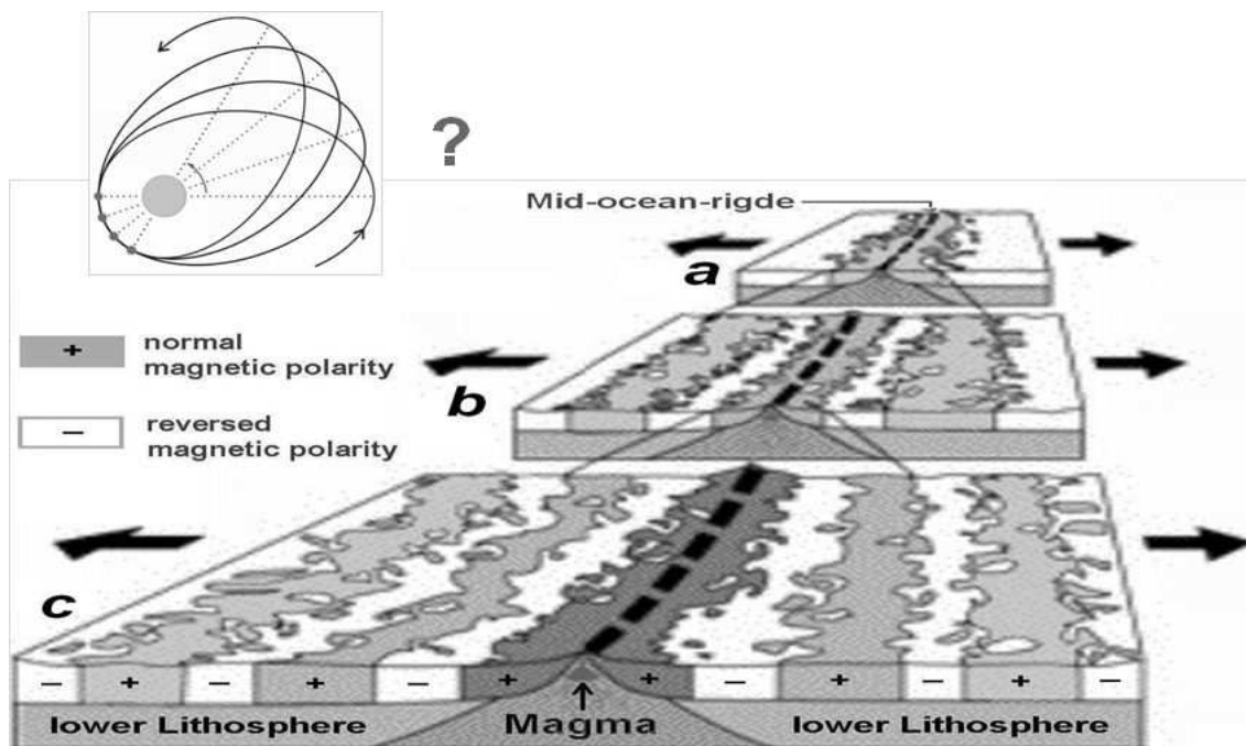
Fig. 33: Symmetrical ocean-floor-basalts show repeated changes of magnetic polarity.
