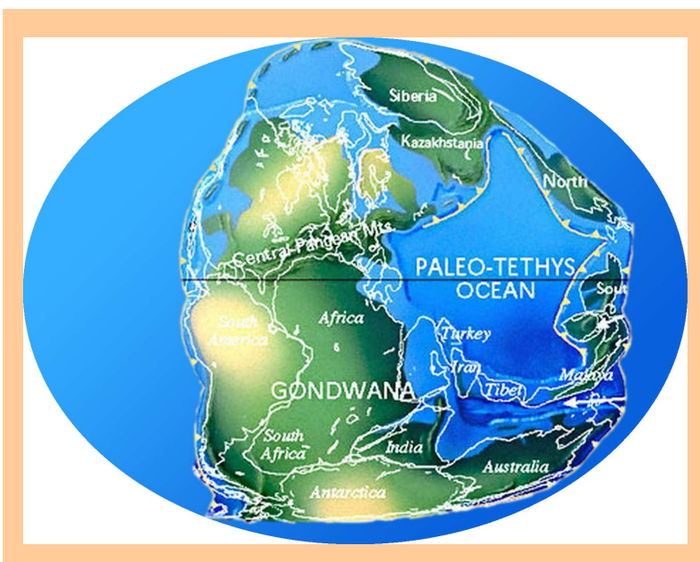
Fig. 6: Paleomap Scotese (2003): Permian: High global temperature.
