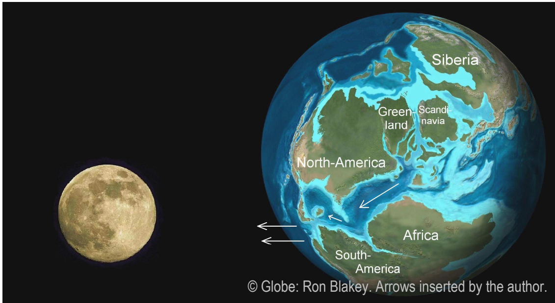
Fig. 11: The earth in Jurassic: The former pathway of the moon is visible (arrows).
