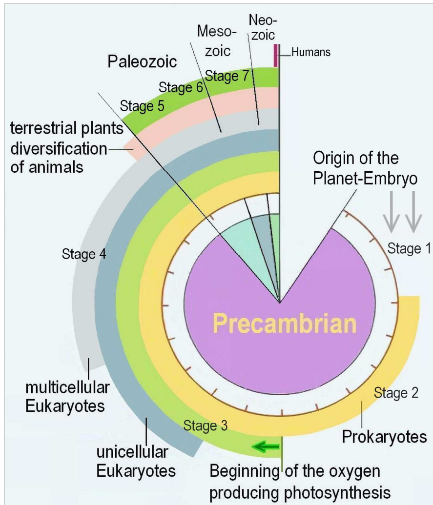
Fig. 3: Timescale of early evolution and biodiversification.
