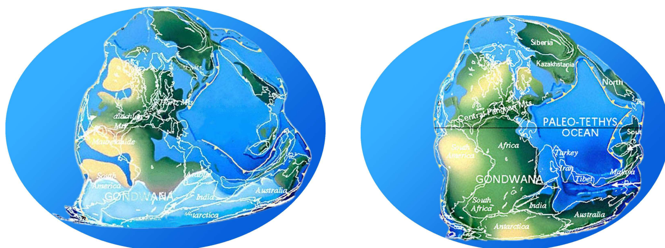
Fig. 5 and 6: Paleomap Scotese (2003): Late Carboniferous (left) and Permian (right)
