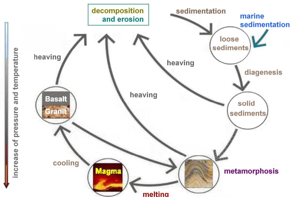
Fig. 4: The cycle of rocks begins with marine biogenic sediments.
